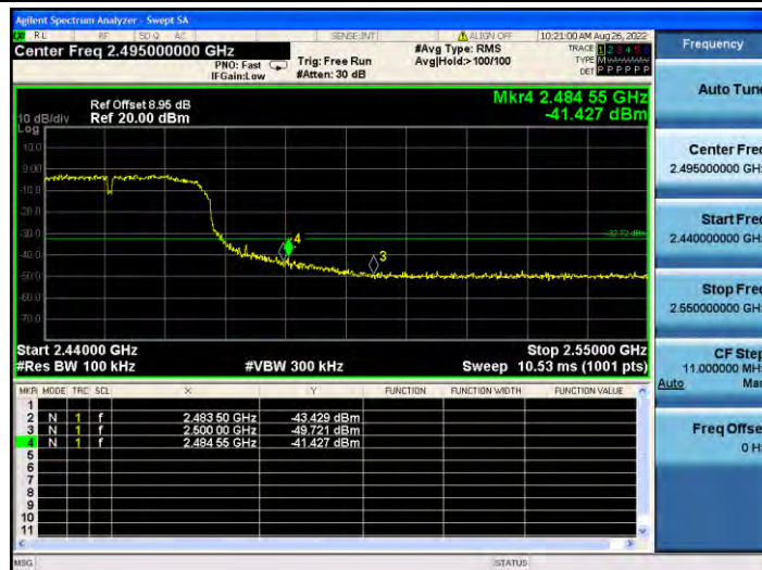
11N40SISO_Ant1_High_2452
