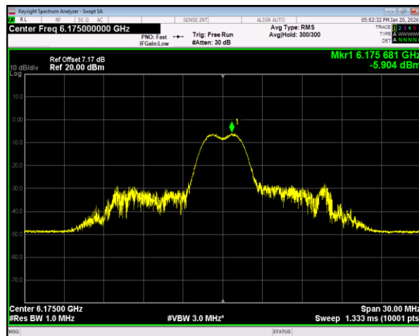
PSD ax20 26@4 6175MHz
