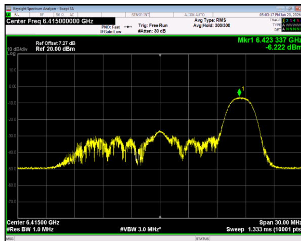
PSD ax20 26@8 6415MHz
