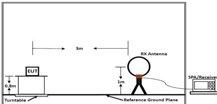
Below 30MHz
