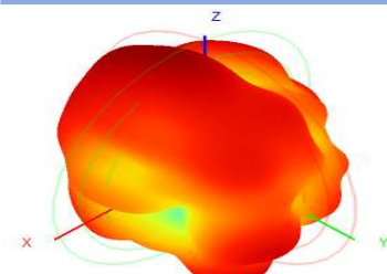
5800.0MHz H+V, Eff: 49.78% / Gain: 2.
