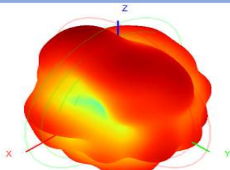
5550.0MHz H+V, Eff: 52.17% / Gain: 2.15
