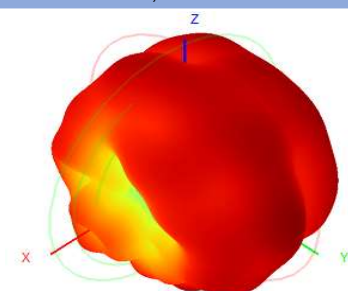
5150.0MHz H+V, Eff: 48.84% / Gain: 2.15
