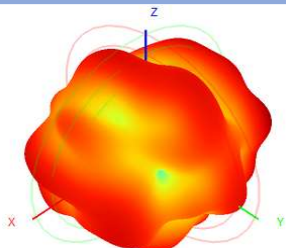
5150.0MHz H+V, Eff: 48.84% / Gain: 2.15
