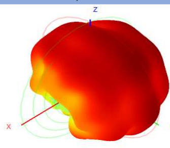
5550.0MHz H+V, Eff: 52.17% / Gain: 2.15
