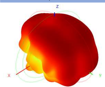
5800.0MHz H+V, Eff: 49.78% / Gain: 2.
