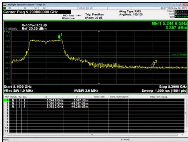
802.11n40Right Side
