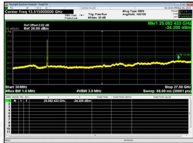
802.11n40 on channel 40
