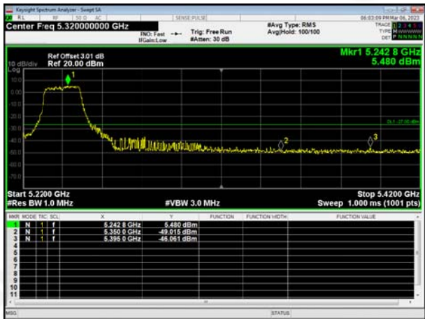
802.11n20Right Side
