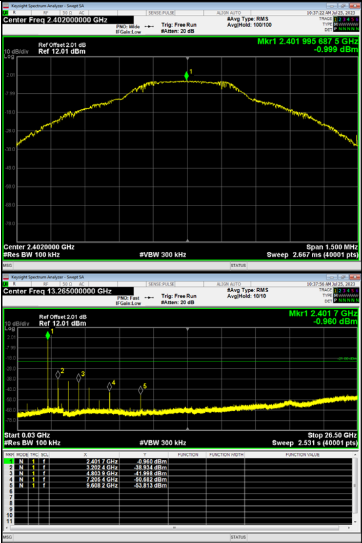
30MHz~26.5GHz
