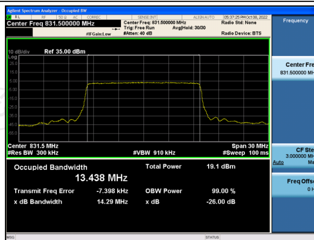
Band26-15MHz-QPSK-26915-75RB#0
