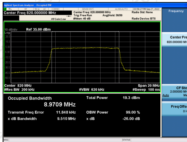
Band18-10MHz-16QAM-23925-50RB#0
