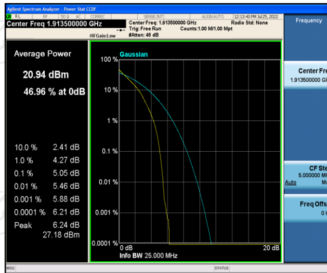
Band25-3MHz-16QAM-26055-1RB#0
