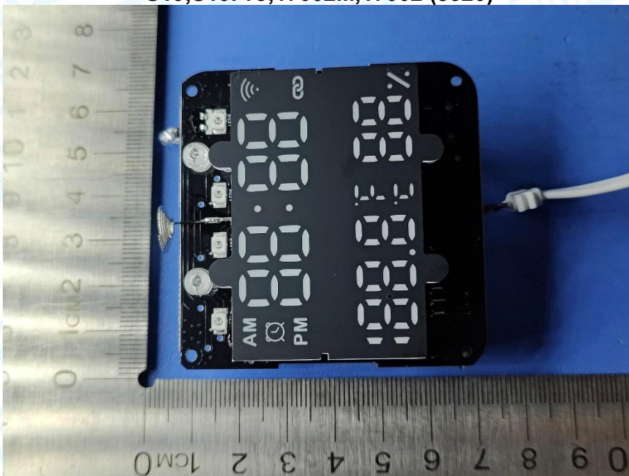
Photo 10 Appearance of PCB S19,S19Pro,17002M,17002 (8320)
