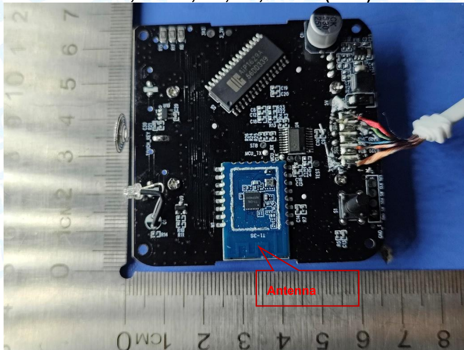
Photo 12 Appearance of PCB S09,S09Pro,S16,S17,S17Pro (8310)
