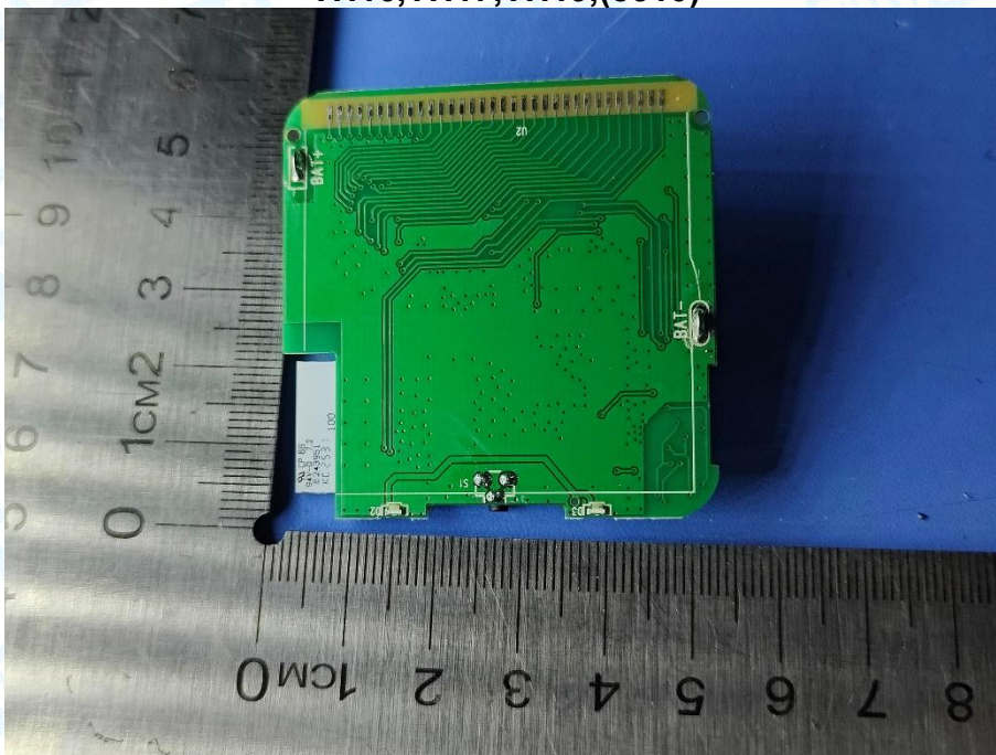
Photo 17 Appearance of PCB TH16,TH17,TH19,(8310)
