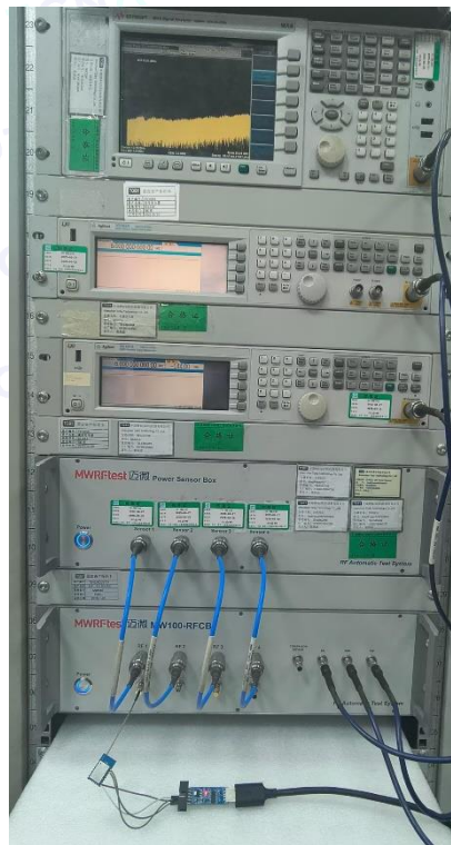
Photo of Setup for RF Conducted
