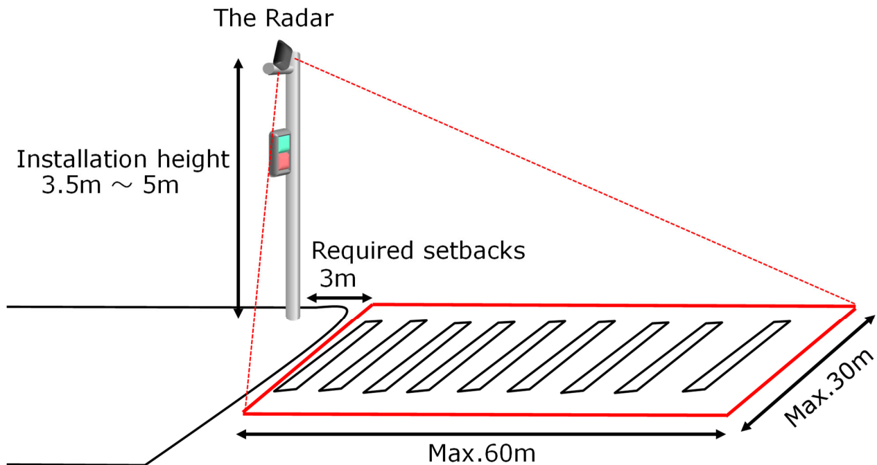
Figure 2. Installation requirement
