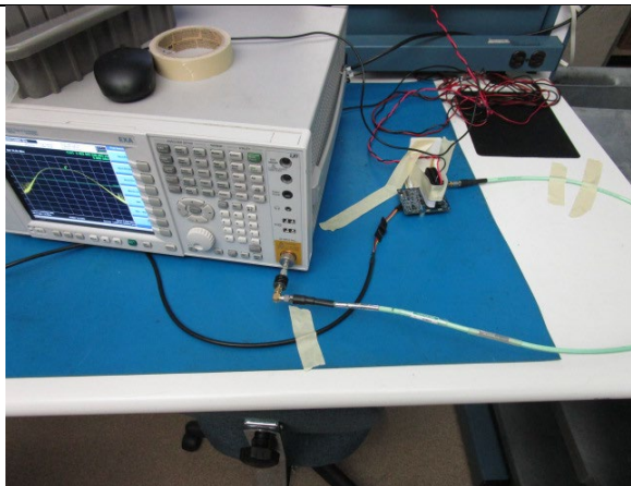
Conducted Setup
