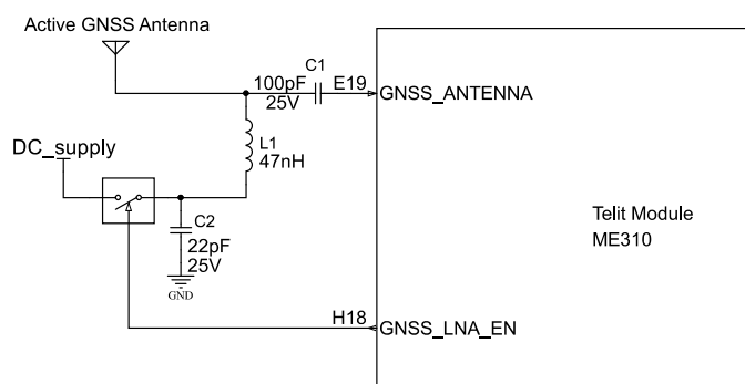
Figure 23: External antenna bias circuitry example
