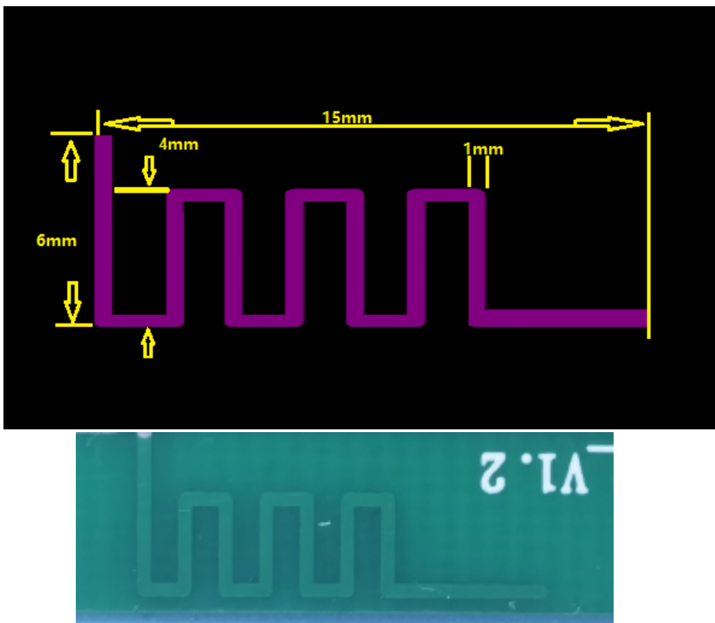
Picture of Antenna
