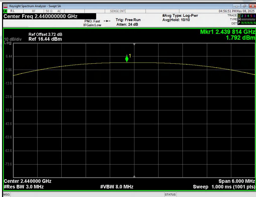
Peak_Output_Power_&_EIRP_NVNT_ANT1_1Mbps_2440
