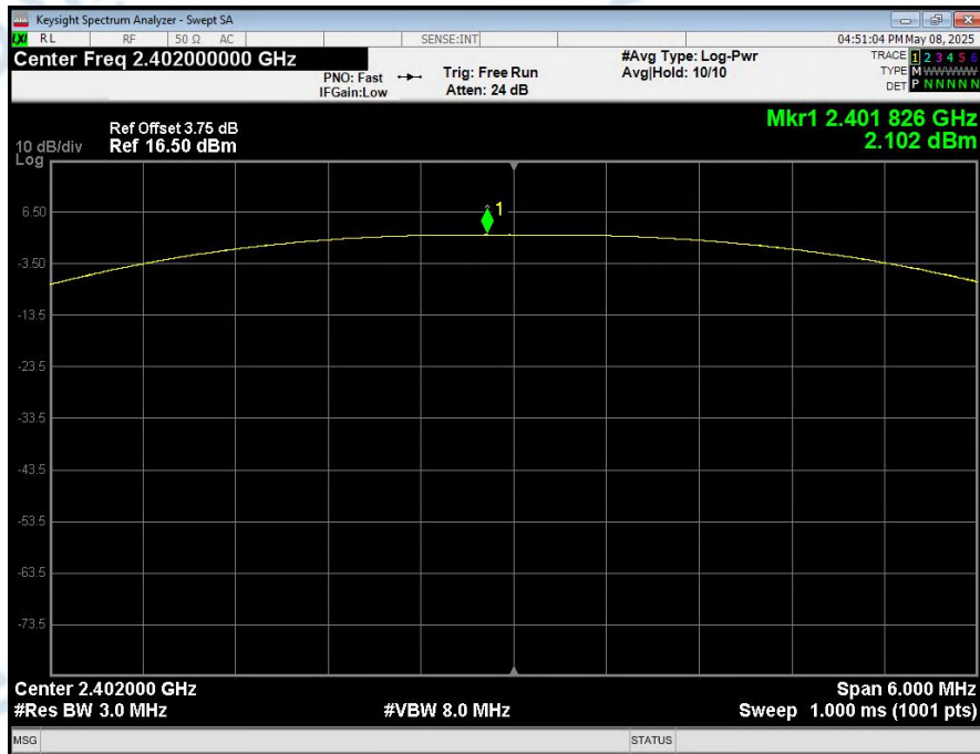
Peak_Output_Power_&_EIRP_NVNT_ANT1_1Mbps_2402
