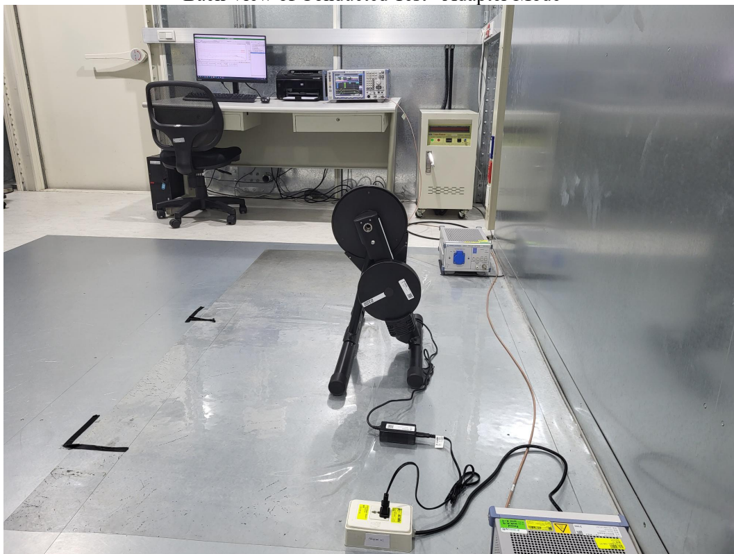
Back View of Conducted Test - Adapter Mode
