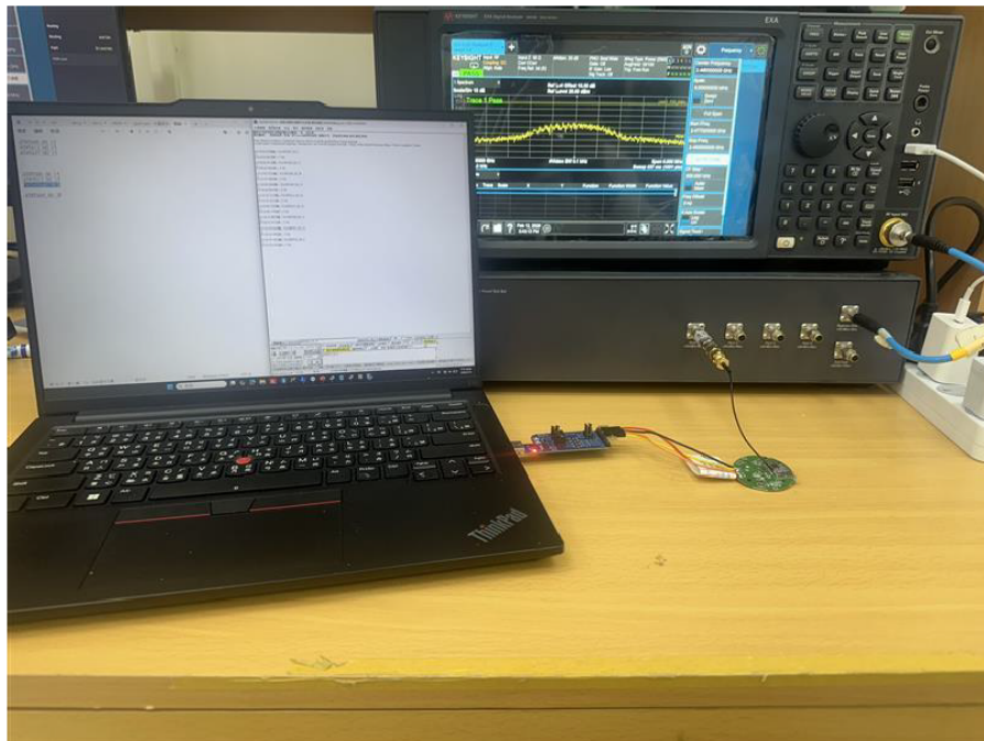
Set-up for Conducted Rear View
