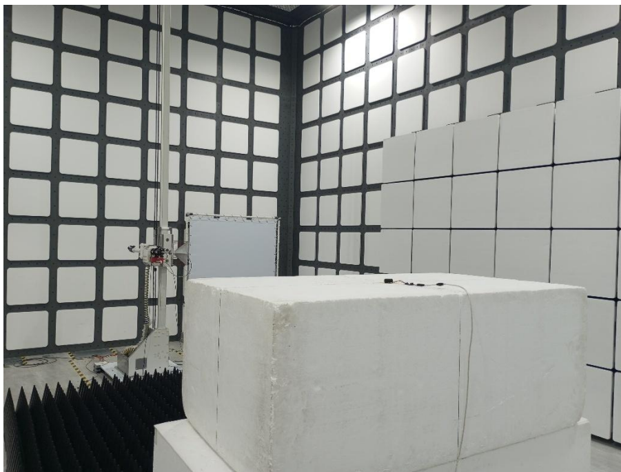
Set-up for Spurious Emissions 1000MHz-18000MHz Rear View
