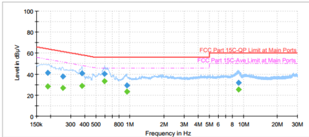
Full Spectrum
