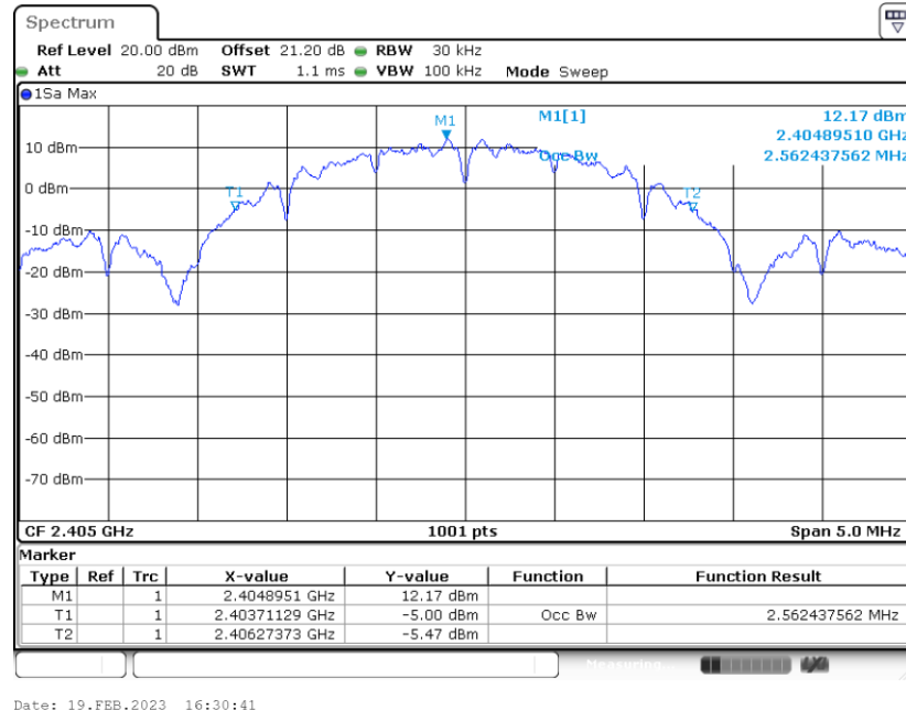
99% Occupied Bandwidth Plot on Channel 11
