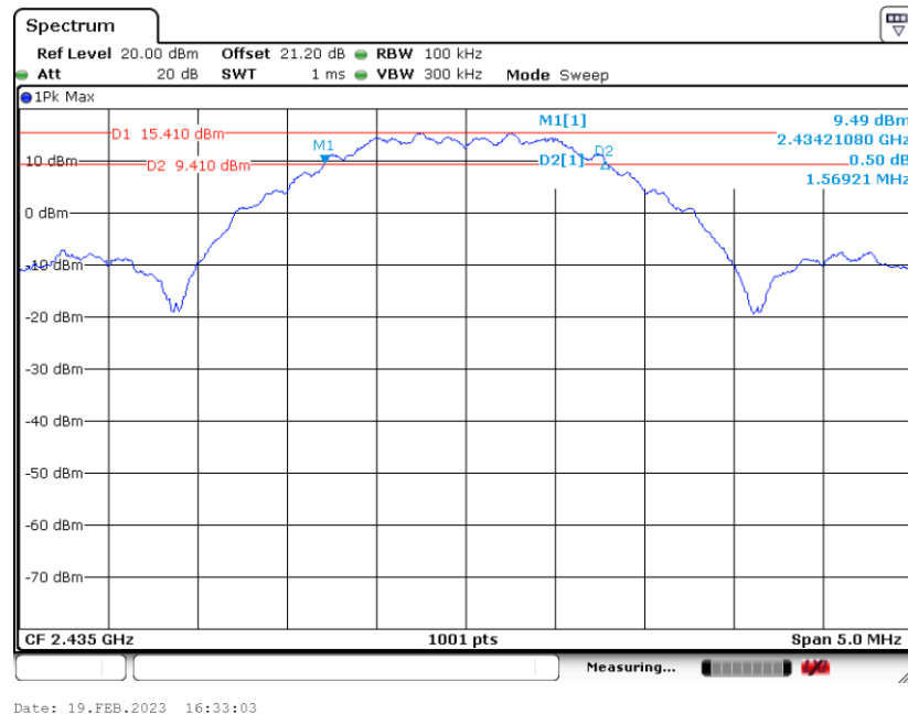
6 dB Bandwidth Plot on Channel 17
