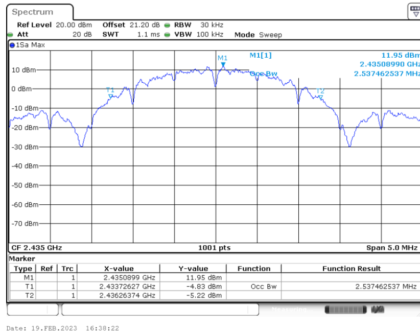
99% Occupied Bandwidth Plot on Channel 17
