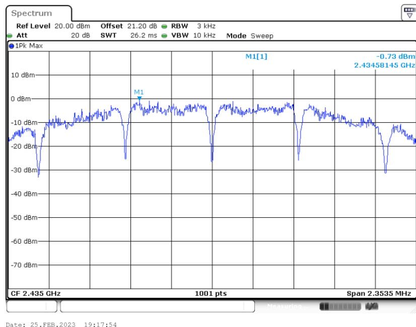
PSD 3kHz Plot on Channel 17
