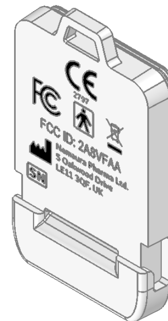
ISOMETRIC VIEW
