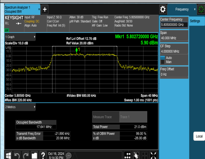
11AC20SISO-Ant2-5805
