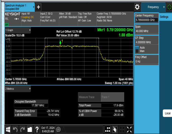
11AC20MIMO-Ant1-5785
