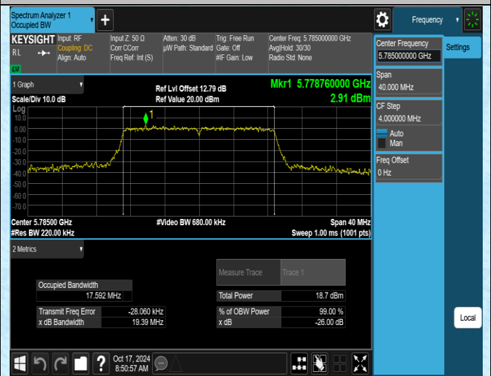
11AC20MIMO-Ant2-5785
