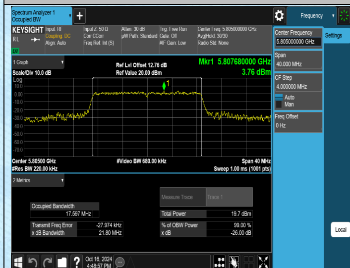
11AC20SISO-Ant1-5805
