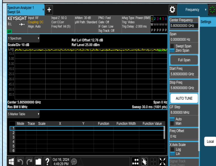
NTNV-11AC20SISO-Ant1-5805
