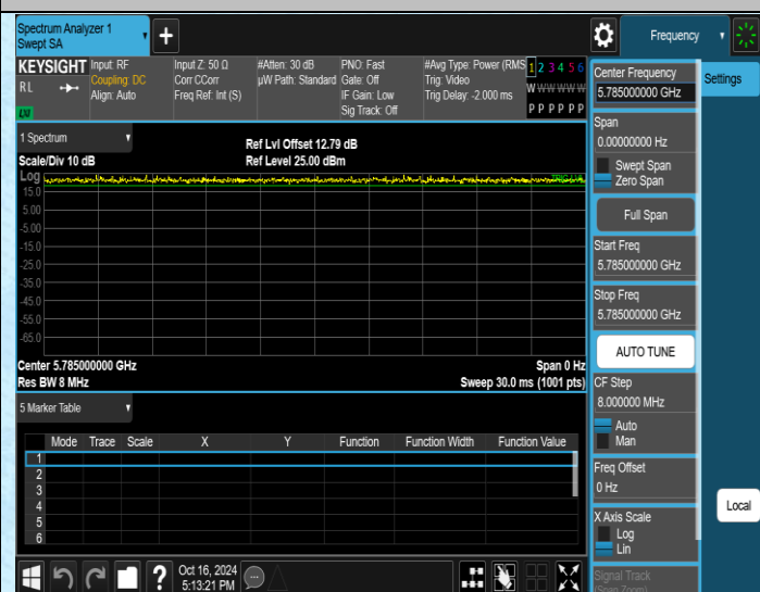
NTNV-11AC20SISO-Ant2-5785
