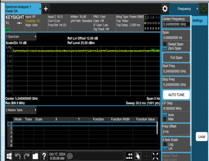
NTNV-11AC20MIMO-Ant2-5240
