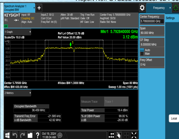
11AC40SISO-Ant4-5795
