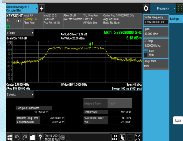
11AC20SISO-Ant3-5785
