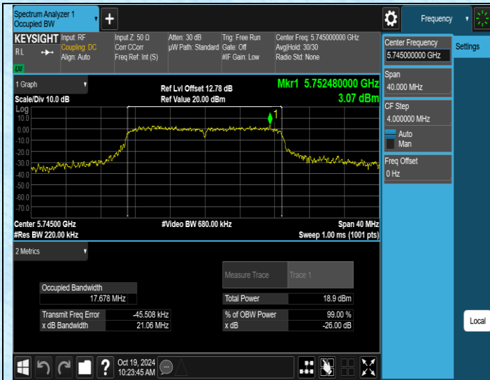
11AC20SISO-Ant3-5745
