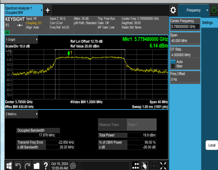
11AC20SISO-Ant4-5785
