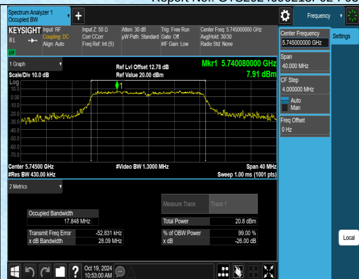
11AC20SISO-Ant4-5745
