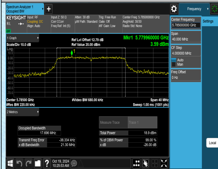
11AC20SISO-Ant3-5785
