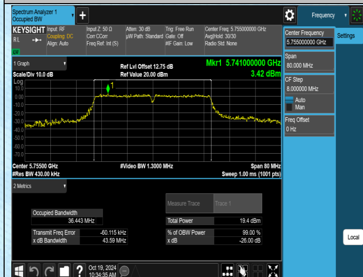
11AC40SISO-Ant3-5755
