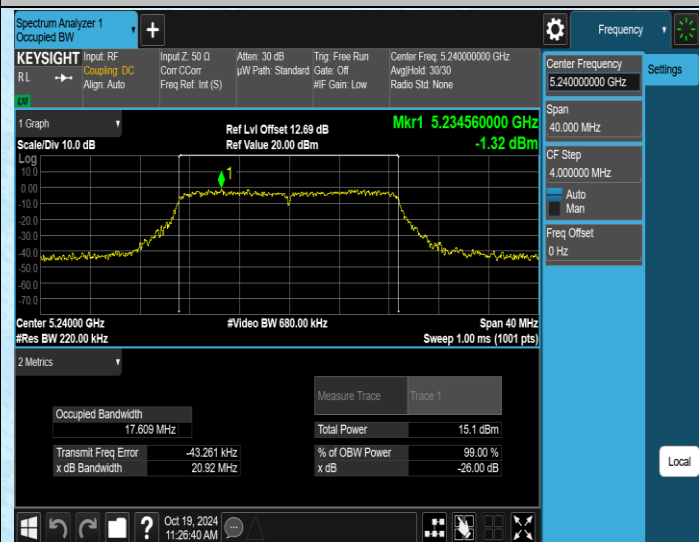
11AC20MIMO-Ant4-5240
