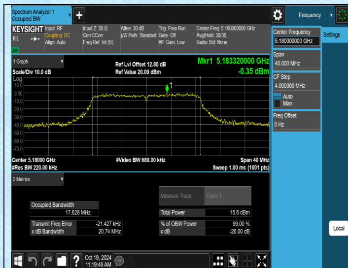
11AC20MIMO-Ant3-5180
