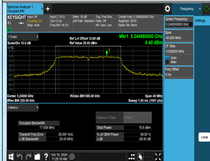
11AC20MIMO-Ant3-5240
