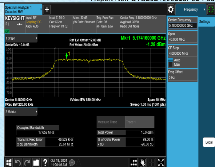
11AC20MIMO-Ant4-5180
