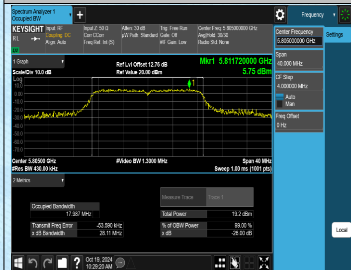
11AC20SISO-Ant3-5805
