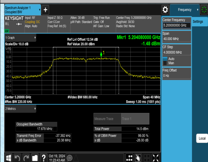
11AC20MIMO-Ant4-5200
