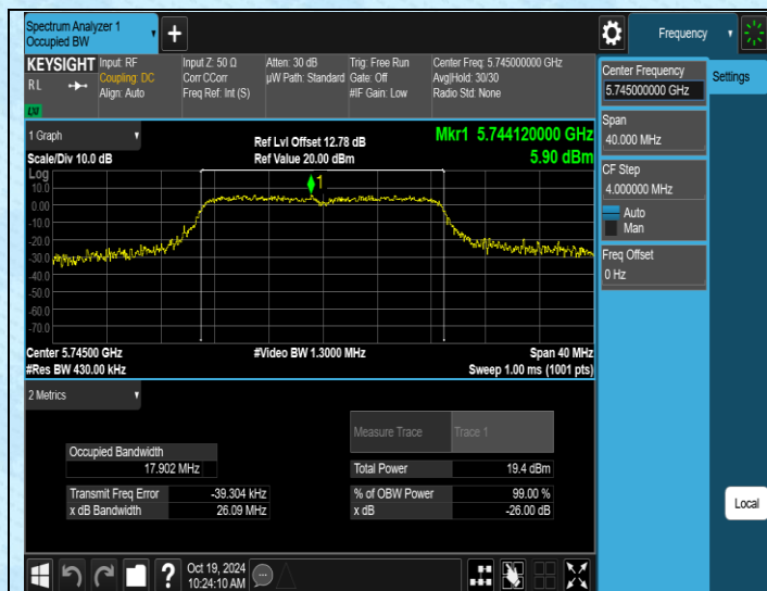
11AC20SISO-Ant3-5745
