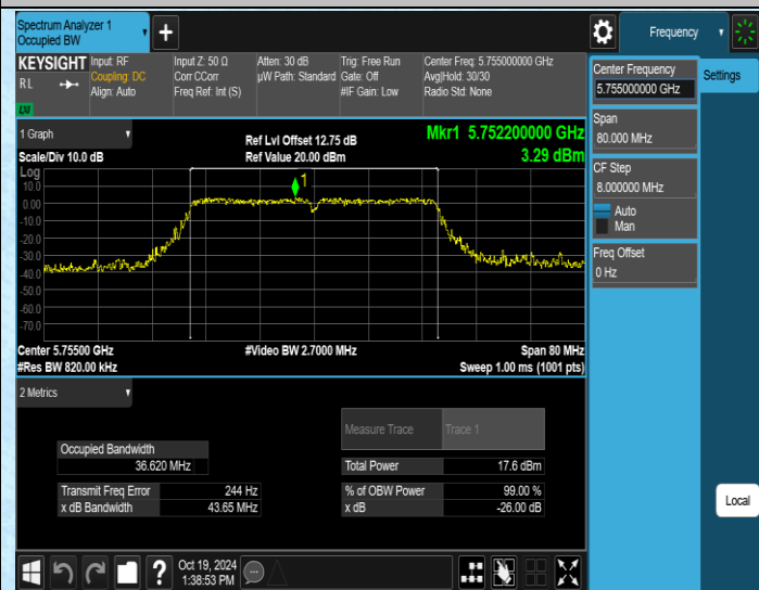
11AC40MIMO-Ant4-5755
