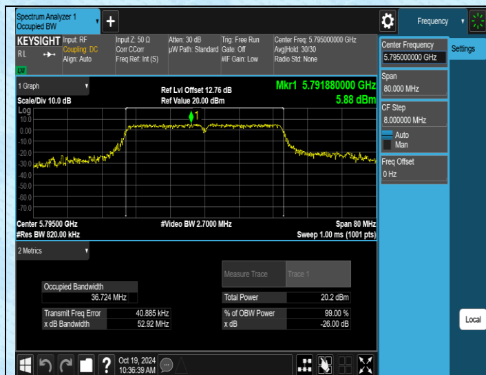
11AC40SISO-Ant3-5795
