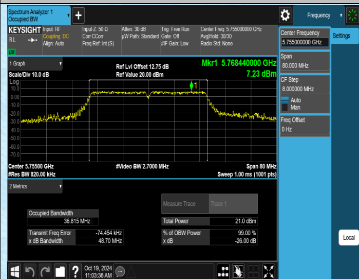
11AC40SISO-Ant4-5755
