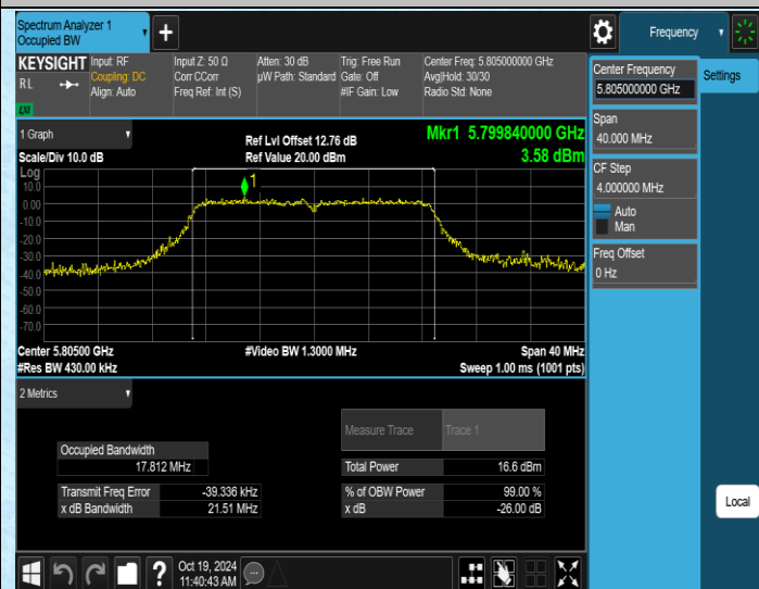
11AC20MIMO-Ant4-5805
