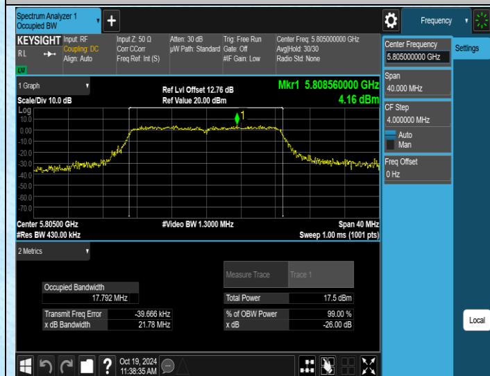
11AC20MIMO-Ant3-5805
