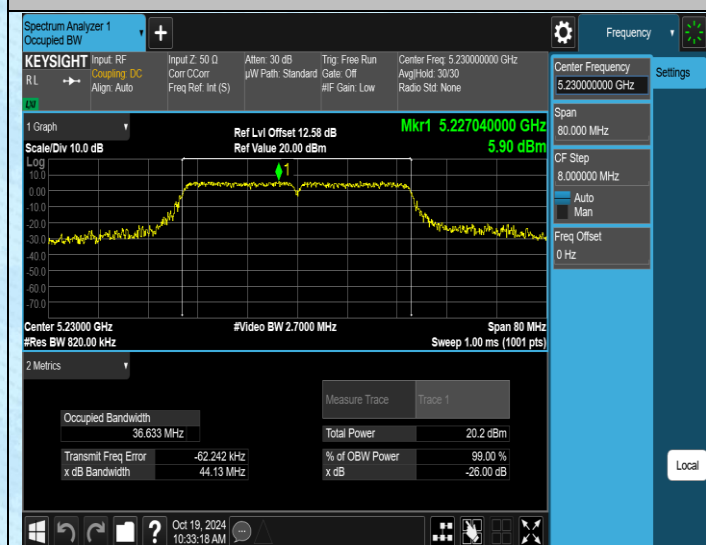
11AC40SISO-Ant3-5230
