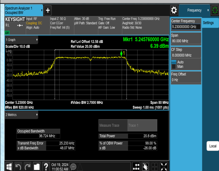
11AC40SISO-Ant4-5230
