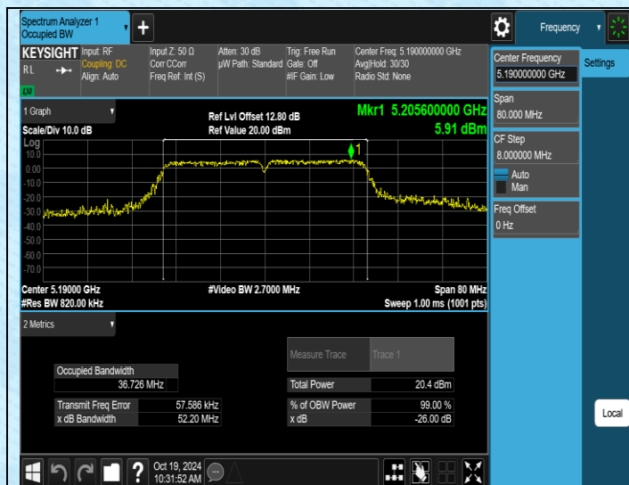
11AC40SISO-Ant3-5190
