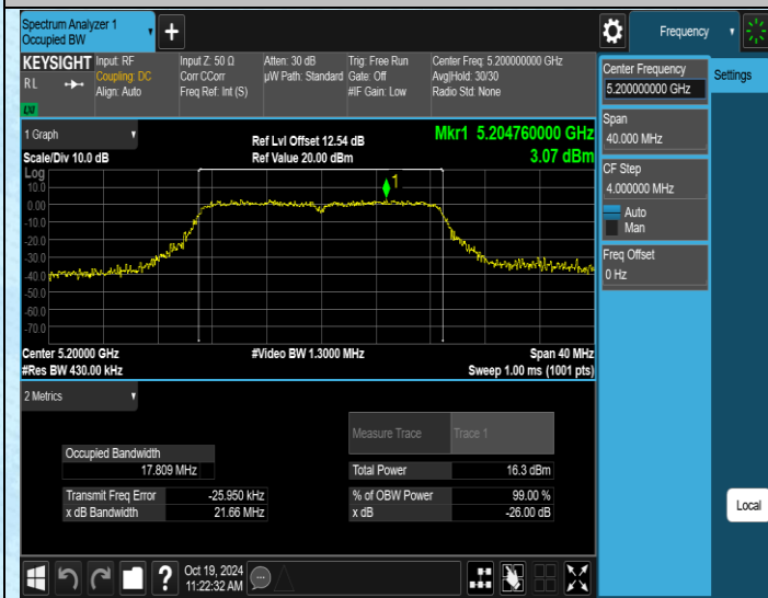
11AC20MIMO-Ant3-5200
