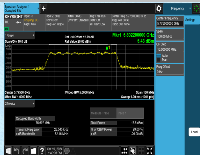
11AC80MIMO-Ant4-5775
