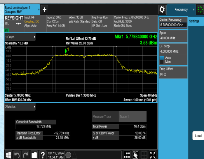
11AC20MIMO-Ant4-5785
