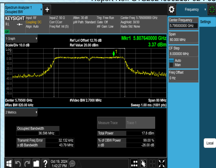
11AC40MIMO-Ant4-5795
