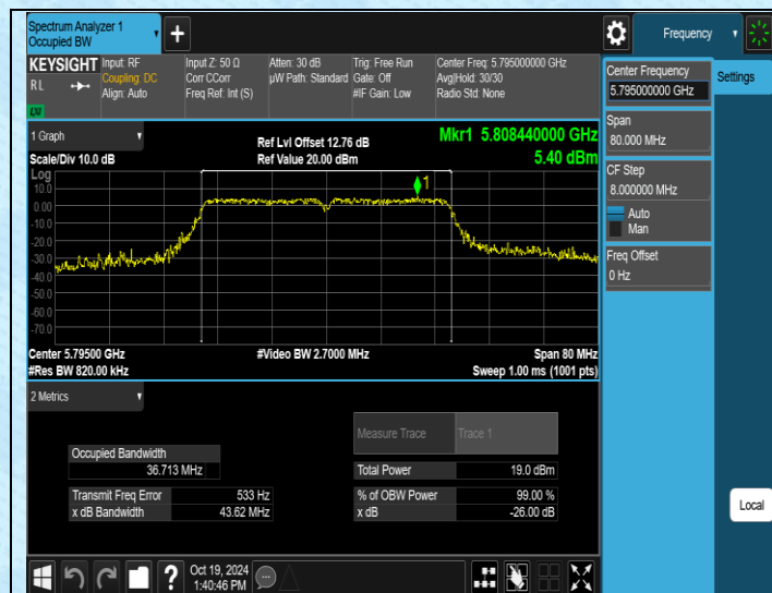
11AC40MIMO-Ant3-5795
