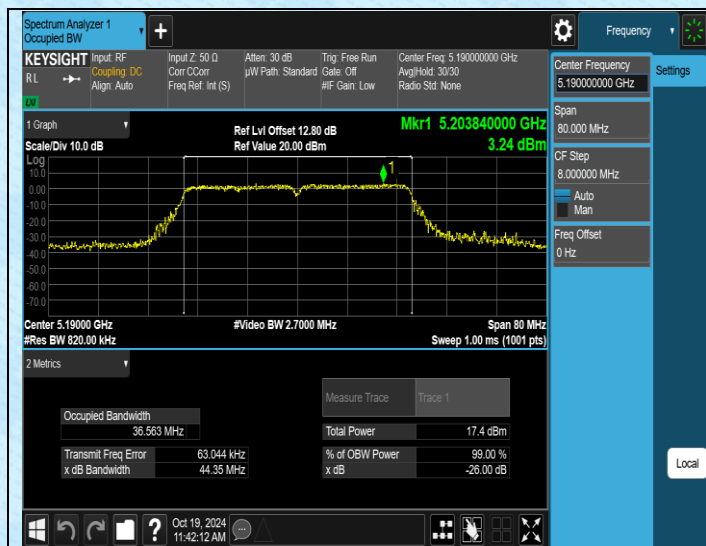
11AC40MIMO-Ant3-5190
