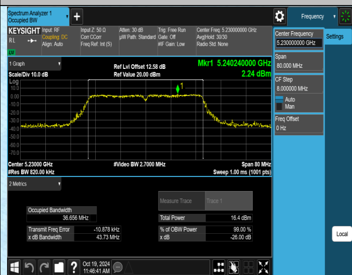
11AC40MIMO-Ant4-5230
