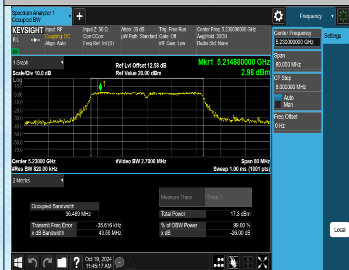
11AC40MIMO-Ant3-5230
