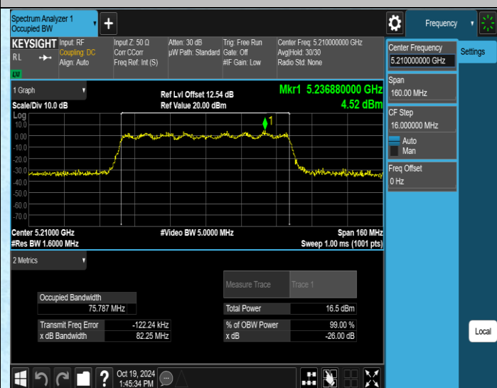
11AC80MIMO-Ant4-5210
