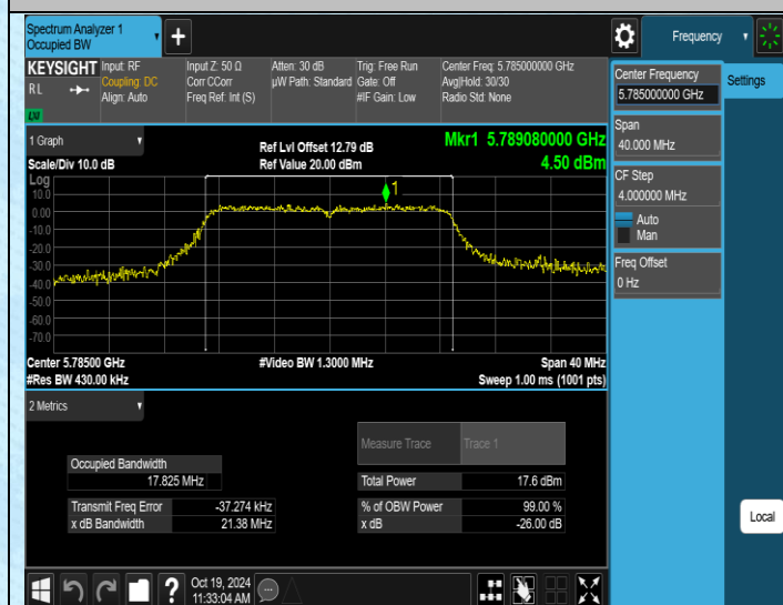
11AC20MIMO-Ant3-5785
