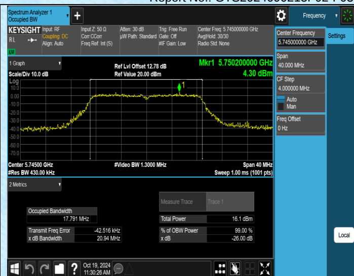
11AC20MIMO-Ant4-5745
