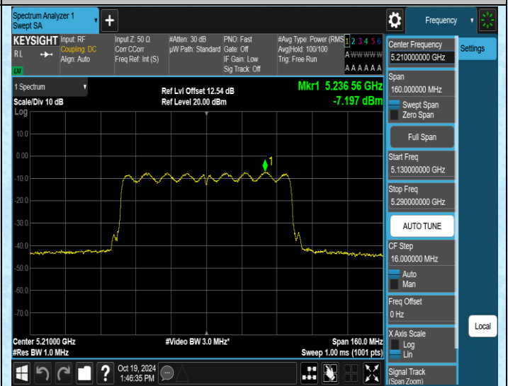
11AC80MIMO-Ant4-5210-PASS
