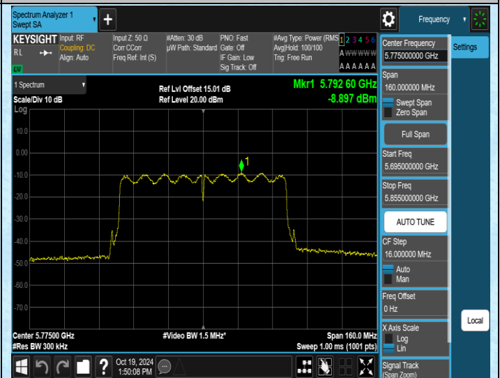
11AC80MIMO-Ant4-5775-PASS
