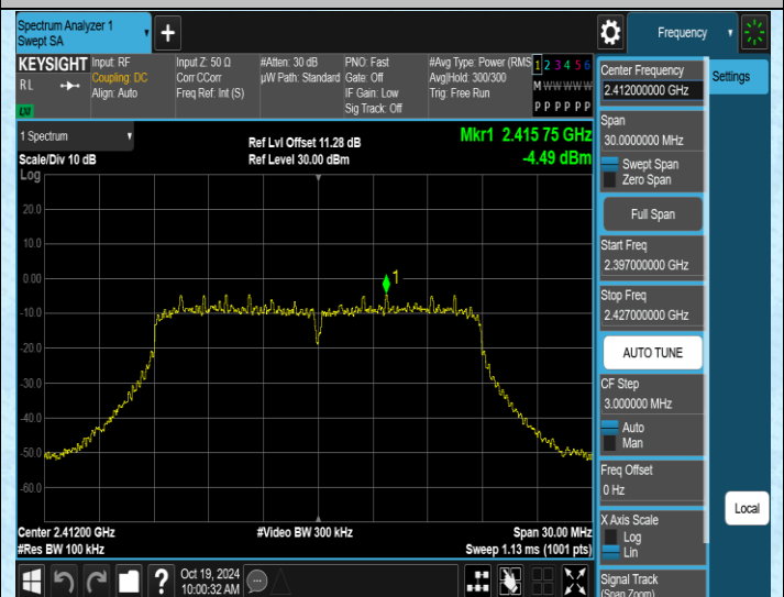
11N20MIMO-Ant4-2412-0~Reference-PASS
