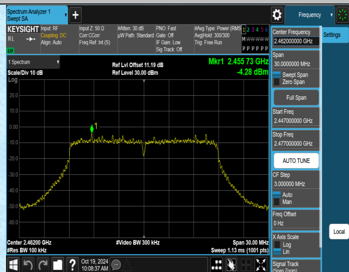
11N20MIMO-Ant4-2462-0~Reference-PASS
