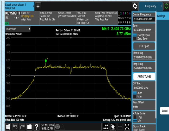
11N20MIMO-Ant3-2412-0~Reference-PASS
