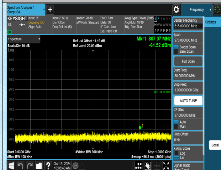
11N20MIMO-Ant4-2462-30~1000-PASS
