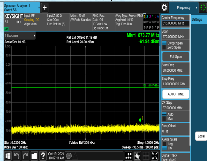
11N20MIMO-Ant3-2462-30~1000-PASS
