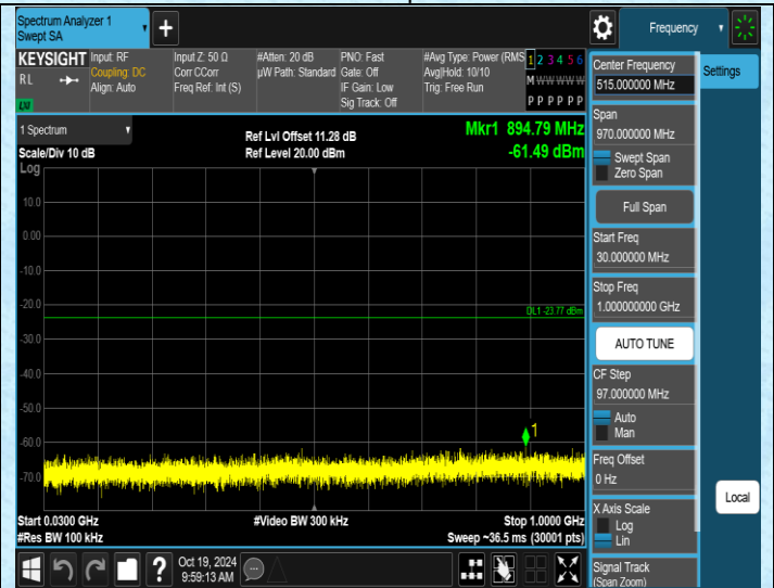
11N20MIMO-Ant3-2412-30~1000-PASS
