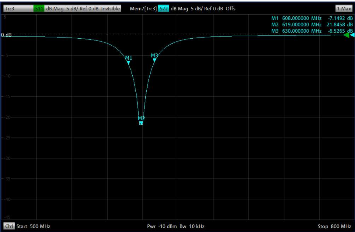
Figure 1 Return loss
