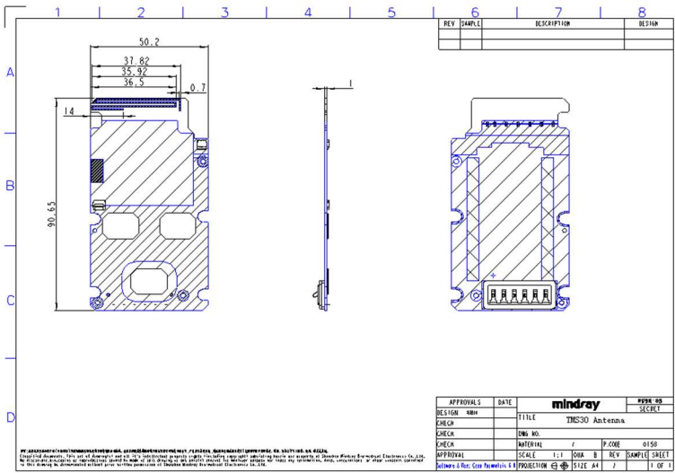
Figure 10 structure drawing
