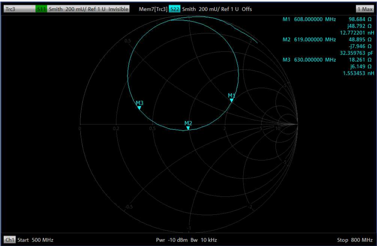
Figure 3 Smith Chart
