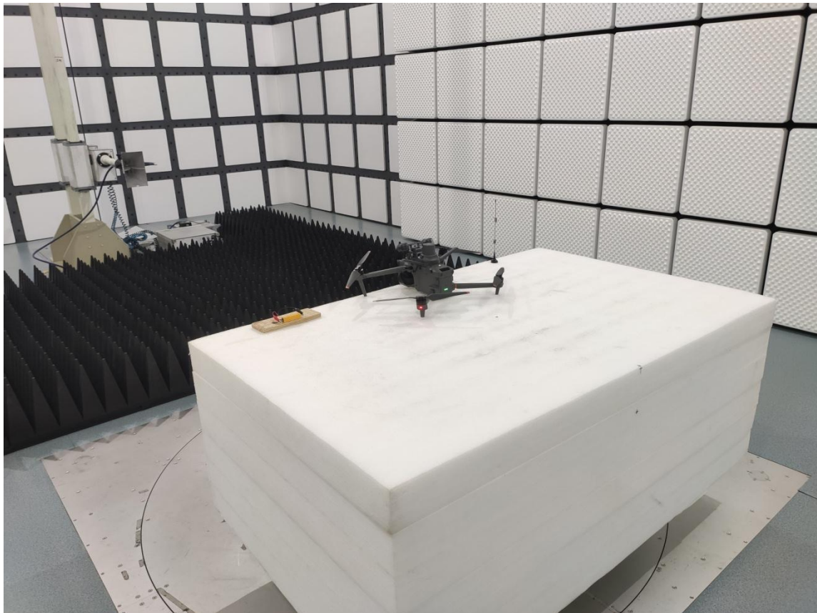
Radiated Emissions Test View (Above 1GHz)
