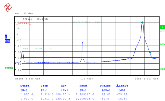
Band2_15MHz_16QAM_19125_1RB#0
