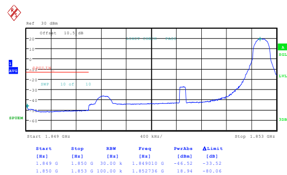
Band2_3MHz_16QAM_18615_1RB#0
