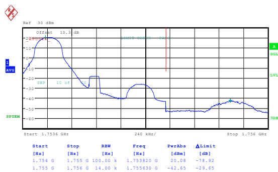
Band4 1.4MHz QPSK 19957 6RB#0
