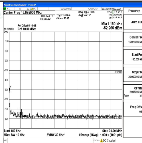
Band2_1.4MHz_QPSK_18607_1RB#0_0.15~30_0.15~30
