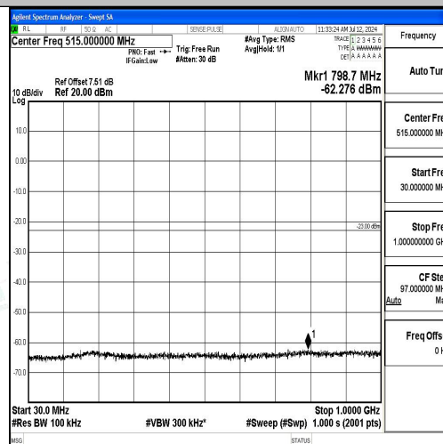
Band2_1.4MHz_QPSK_18607_1RB#0_30~1000_30~1000
