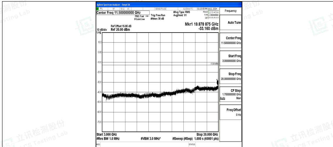
Band2_15MHz_QPSK_18675_1RB#0_3000~20000_3000~20000
