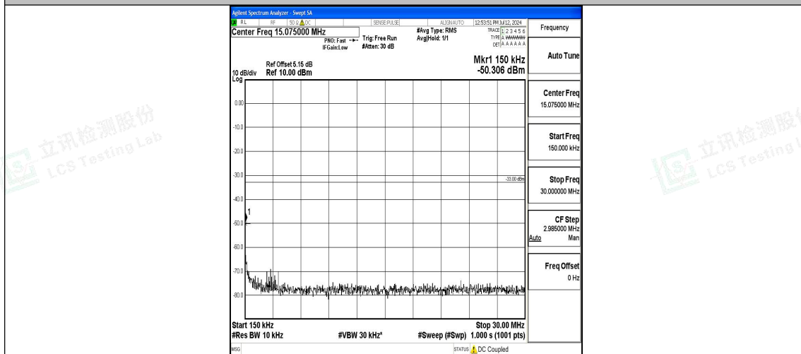
Band2_10MHz_16QAM_18650_1RB#0_0.15~30_0.15~30
