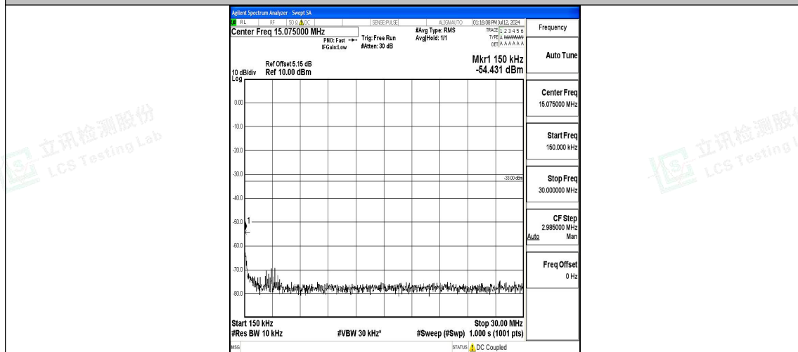
Band2_15MHz_16QAM_18675_1RB#0_0.15~30_0.15~30
