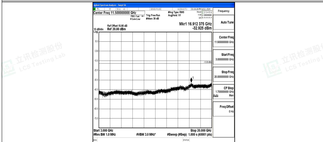
Band2_15MHz_16QAM_18675_1RB#0_3000~20000_3000~20000
