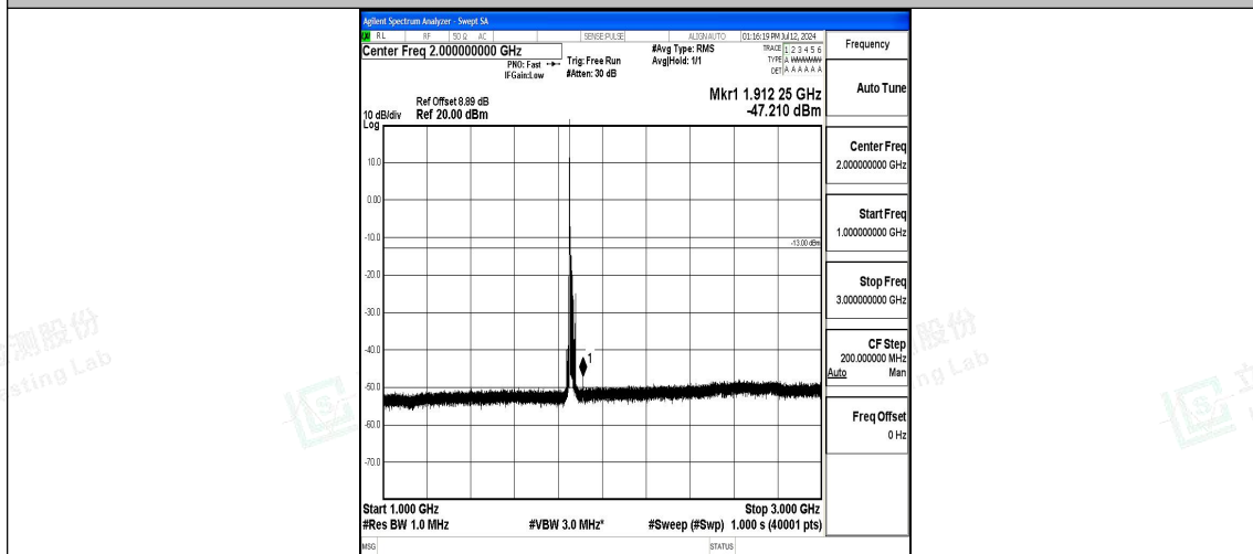
Band2_15MHz_16QAM_18675_1RB#0_1000~3000_1000~3000
