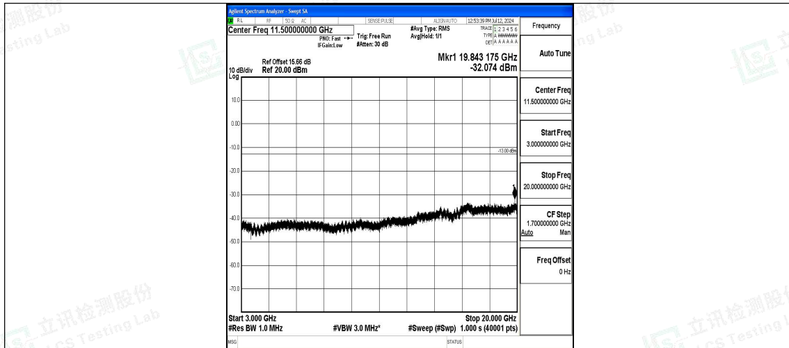
Band2_10MHz_QPSK_18650_1RB#0_3000~20000_3000~20000
