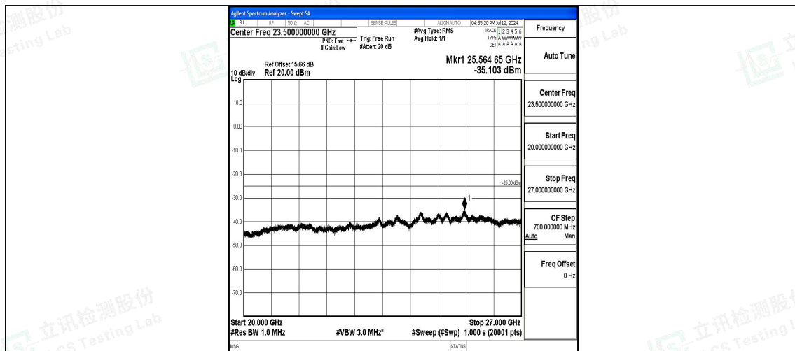
Band7_20MHz_QPSK_21100_1RB#0_20000~27000_20000~27000
