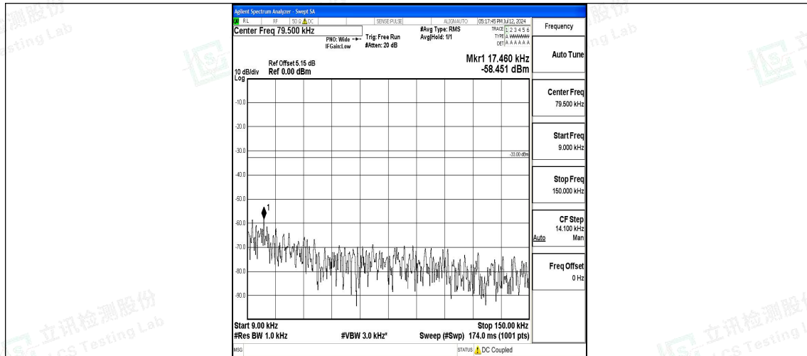
Band17_5MHz_QPSK_23790_1RB#0_0.009~0.15_0.009~0.15
