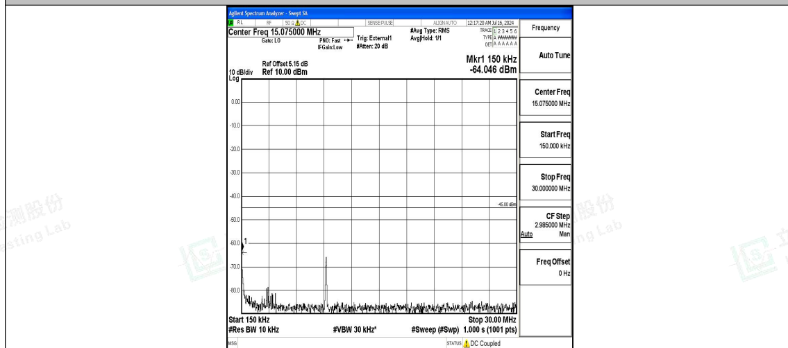
Band38_10MHz_16QAM_37800_1RB#0_0.15~30_0.15~30
