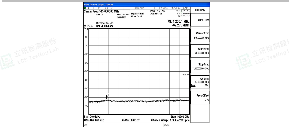
Band38_10MHz_16QAM_37800_1RB#0_30~1000_30~1000
