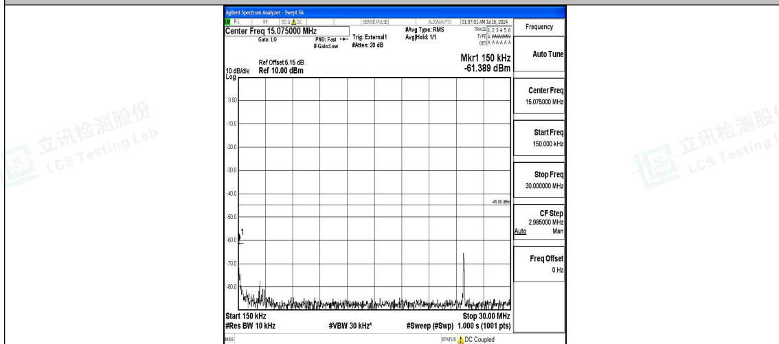
Band38_20MHz_16QAM_38000_1RB#0_0.15~30_0.15~30
