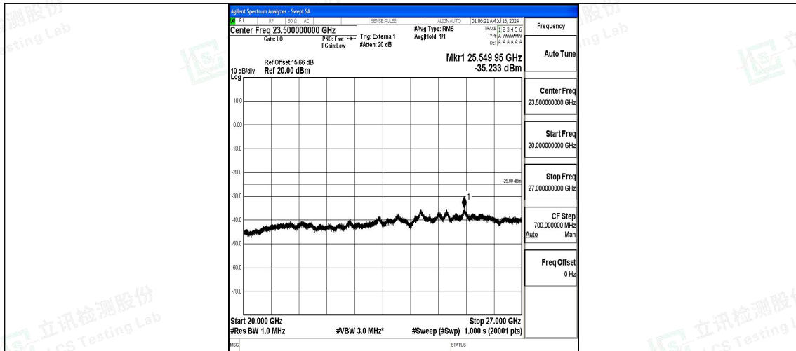
Band38_20MHz_QPSK_38000_1RB#0_20000~27000_20000~27000
