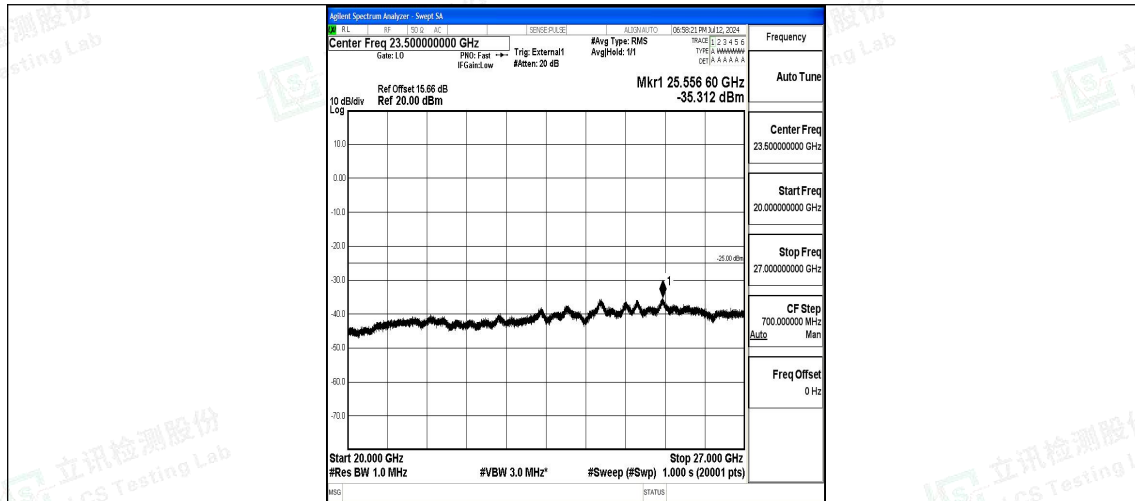
Band41_10MHz_16QAM_41540_1RB#0_20000~27000_20000~27000
