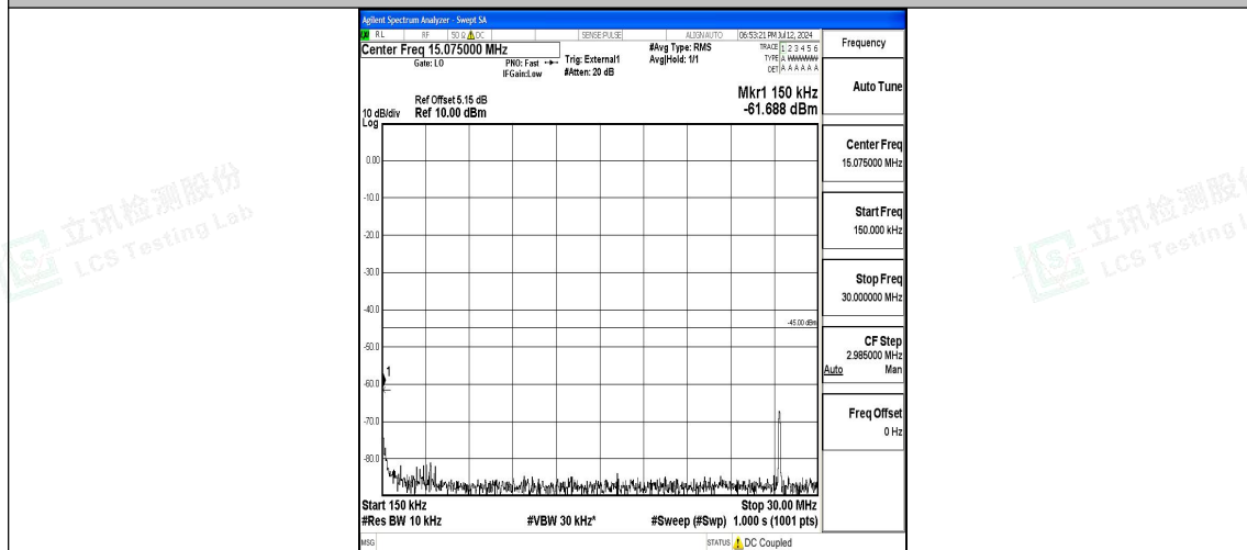
Band41_10MHz_16QAM_40620_1RB#0_0.15~30_0.15~30
