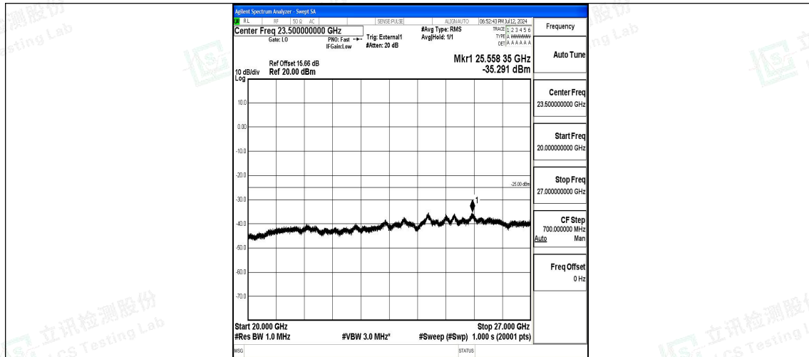
Band41_10MHz_QPSK_40620_1RB#0_20000~27000_20000~27000
