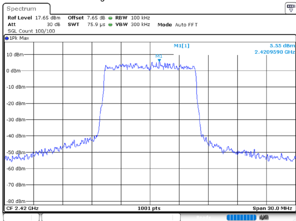
Band Edge NVNT 10M 2420MHz Ant 1 Emission
