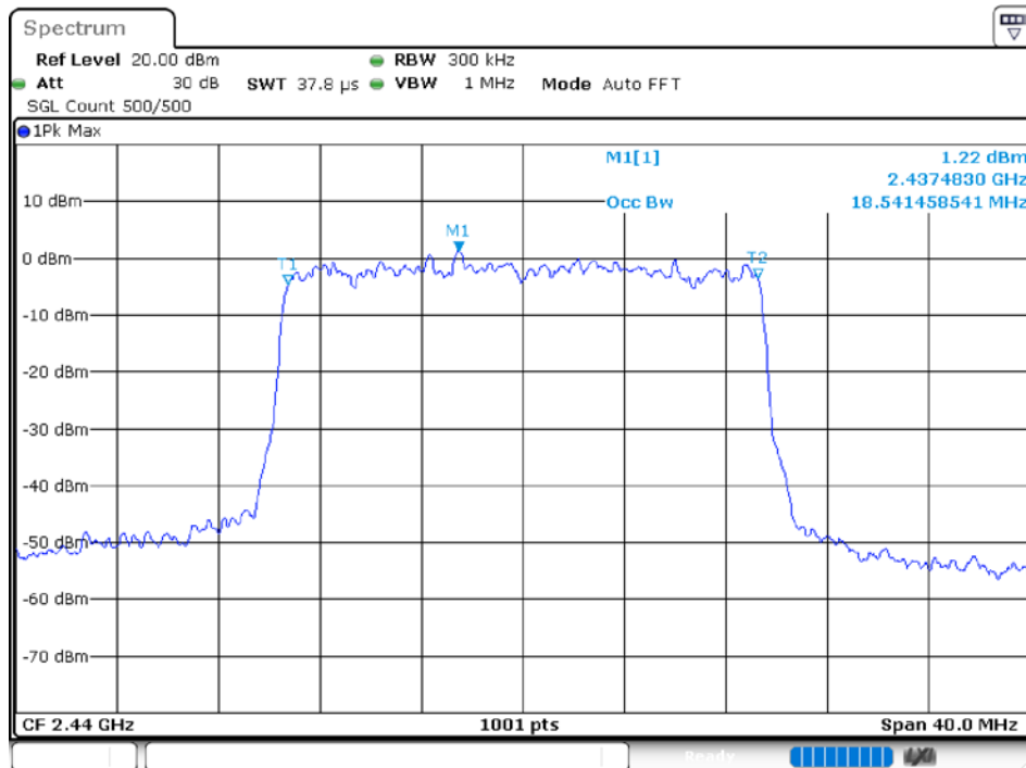
-6 dB BW NVNT 20M 2440MHz Ant 1
