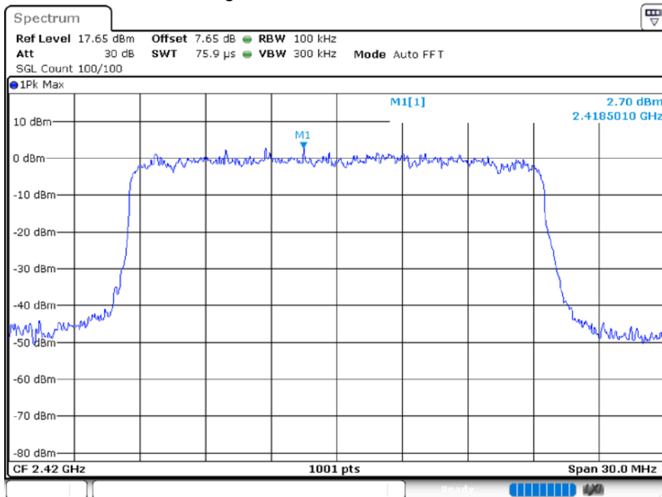
Band Edge NVNT 20M 2420MHz Ant 2 Emission
