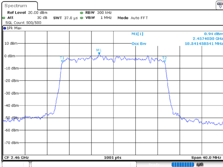
-6 dB BW NVNT 20M 2460MHz Ant 1
