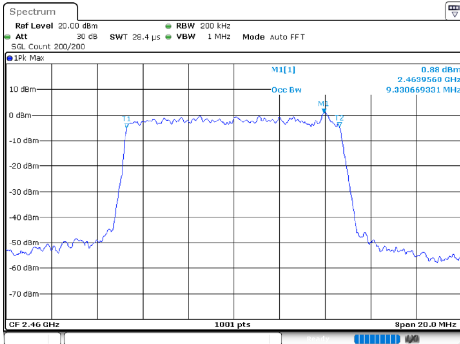
-6 dB BW NVNT 10M 2460MHz Ant 1
