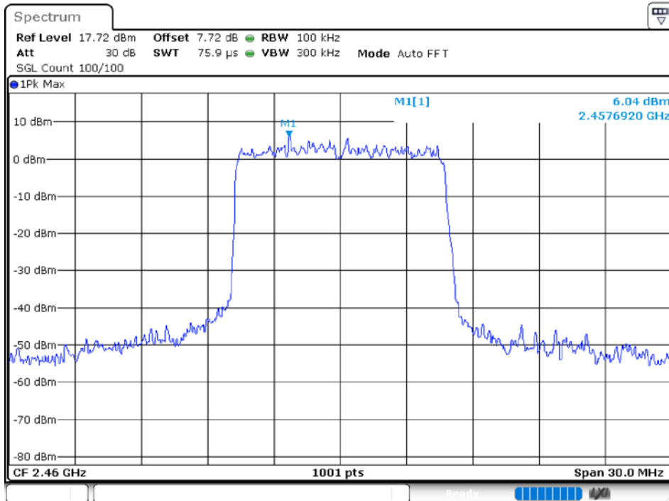
Band Edge NVNT 10M 2460MHz Ant 1 Emission
