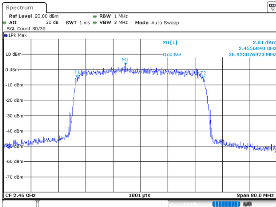
-6 dB BW NVNT 40M 2460MHz Ant 2
