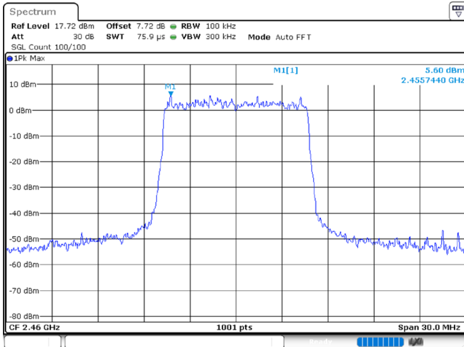
Band Edge NVNT 10M 2460MHz Ant 2 Emission
