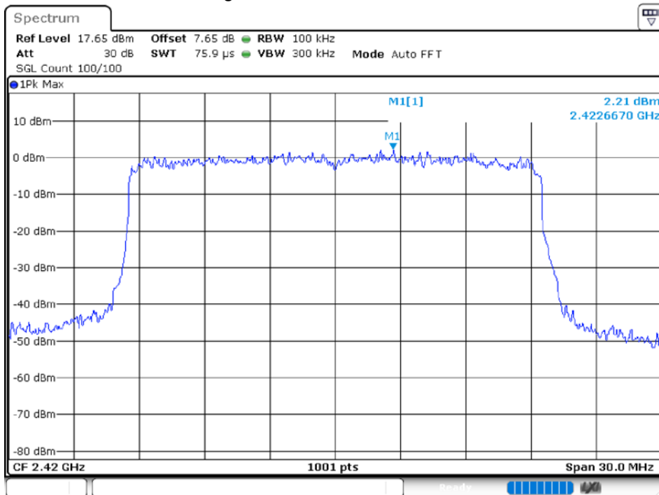
Band Edge NVNT 20M 2420MHz Ant 1 Emission
