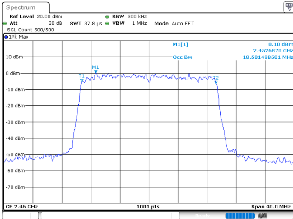
-6 dB BW NVNT 20M 2460MHz Ant 2
