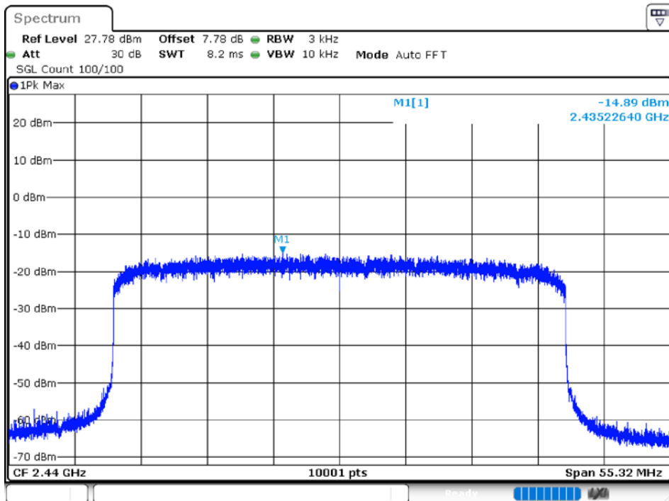
PSD NVNT 40M 2440MHz Ant 2
