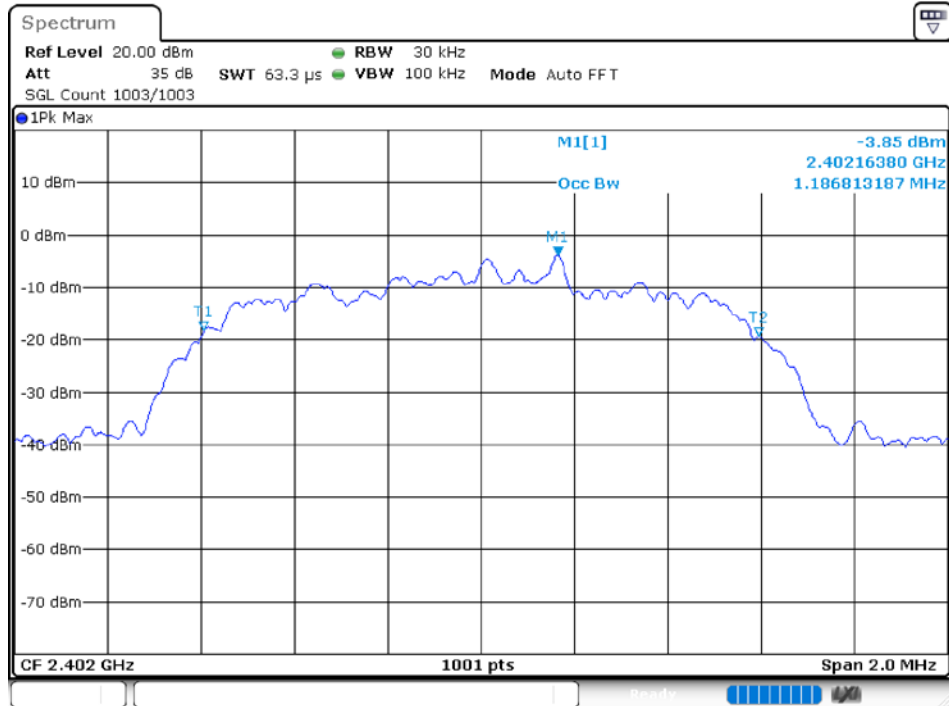
-20 dB BW NVNT 2-DH5 2402MHz Ant1
