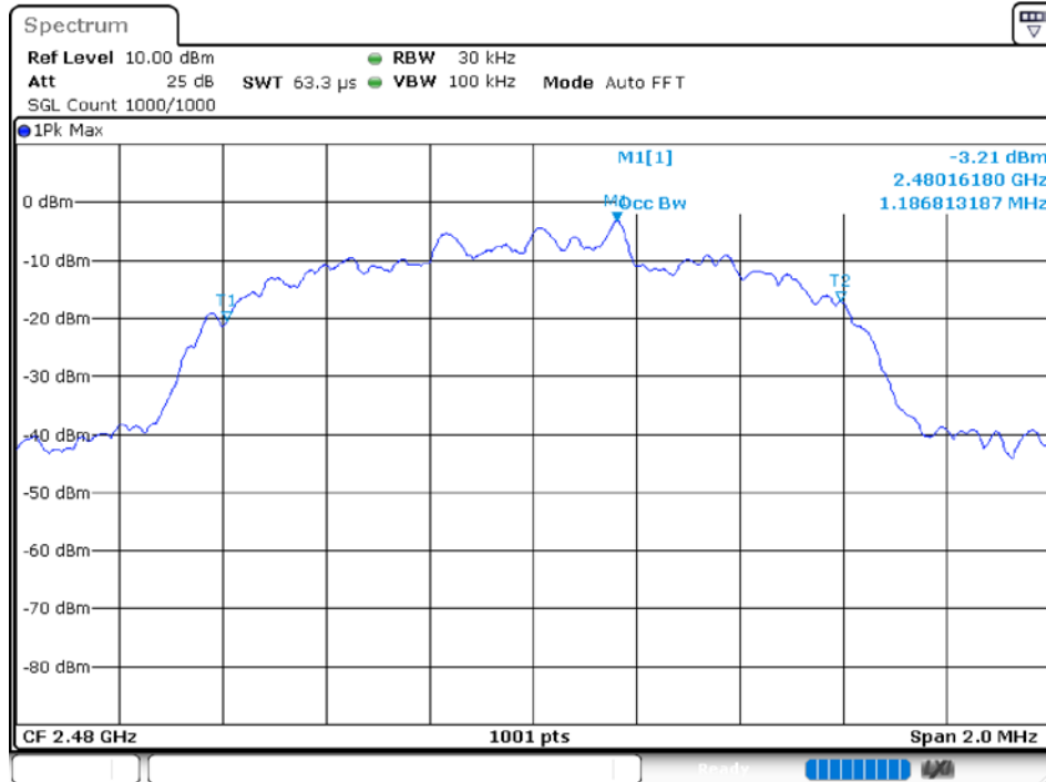
-20 dB BW NVNT 3-DH5 2480MHz Ant1
