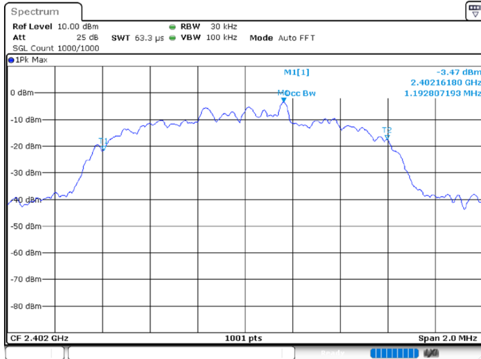
-20 dB BW NVNT 3-DH5 2402MHz Ant1
