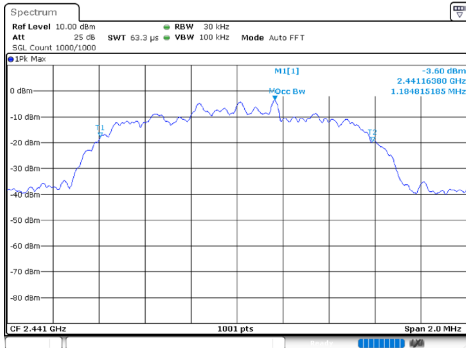
-20 dB BW NVNT 2-DH5 2441MHz Ant1
