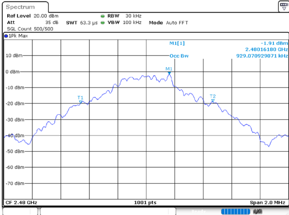
-20 dB BW NVNT 1-DH5 2480MHz Ant1
