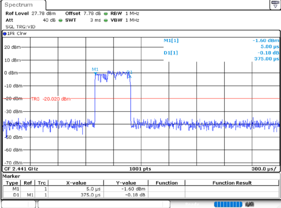
Dwell NVNT 2-DH3 2441MHz
