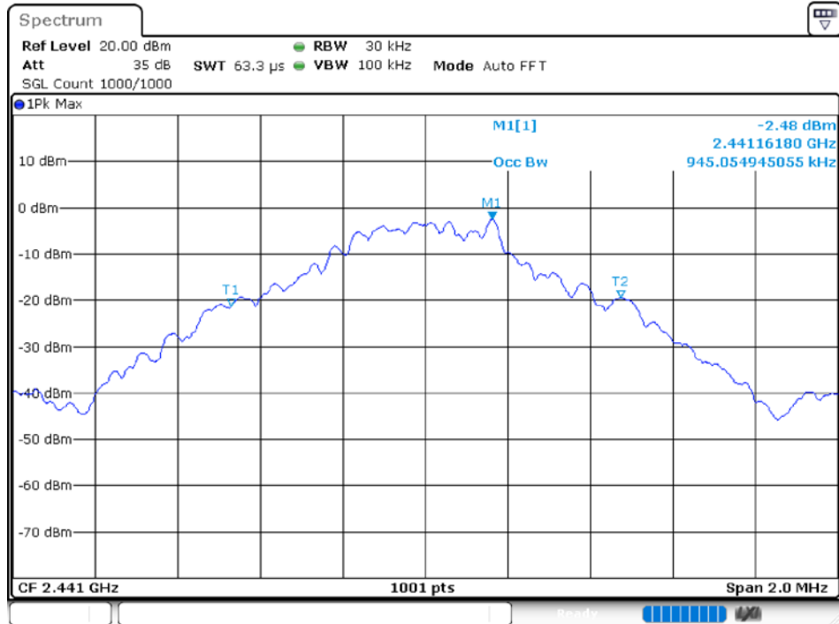
-20 dB BW NVNT 1-DH5 2441MHz Ant1
