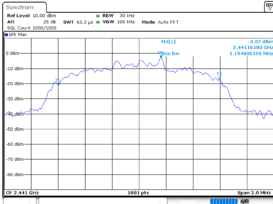
-20 dB BW NVNT 3-DH5 2441MHz Ant1
