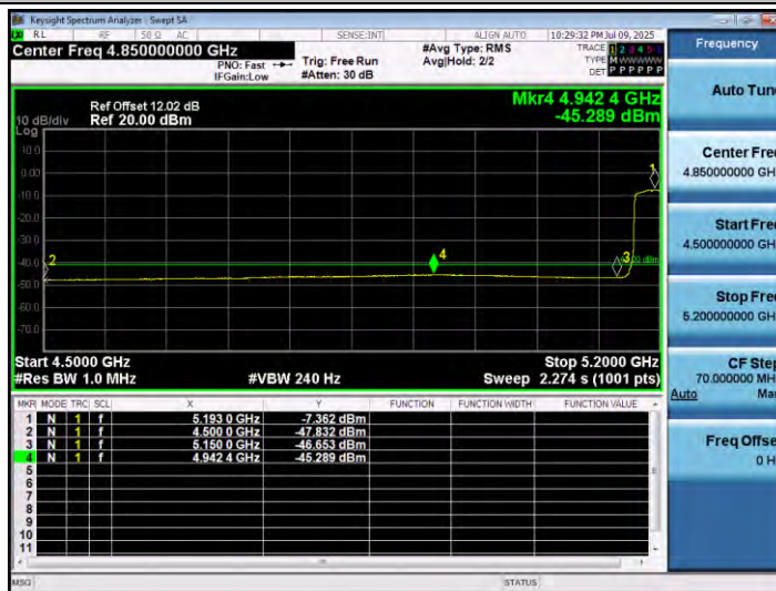
11AX40SISO_Ant2_Low_5190_Peak
