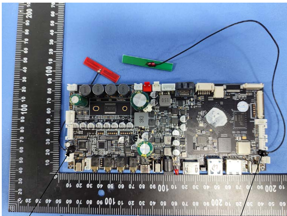
FM Receiver Antenna Location
