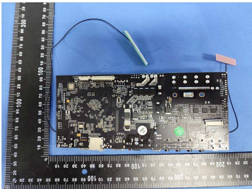
BT Antenna Location
