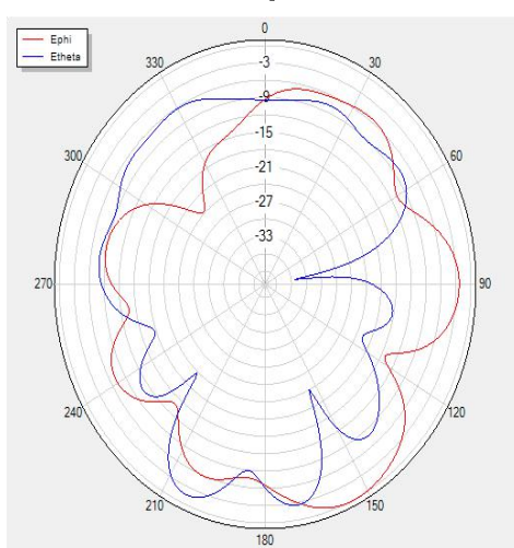
V Phi=0 freq=2430MHz
