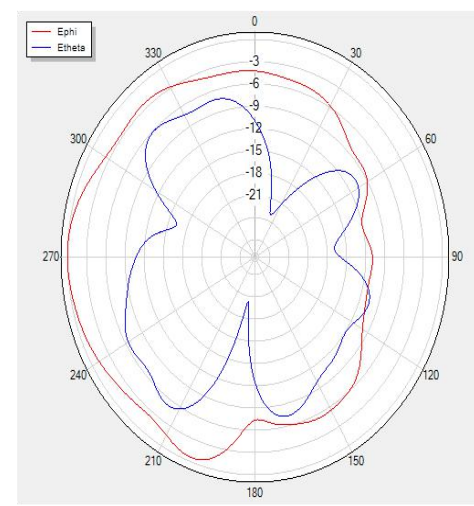
V Phi=90 freq=2500MHz
