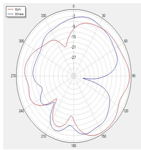
V Phi=0 freq=2490MHz
