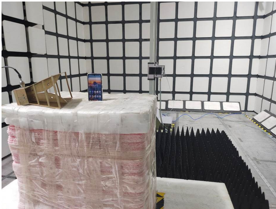
Radiated Emissions View (1-18 GHz)
