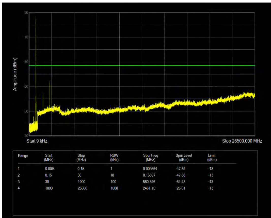
Band18 16QAM BW=5MHz Channel=23925 RB Size=1 Position=#0
