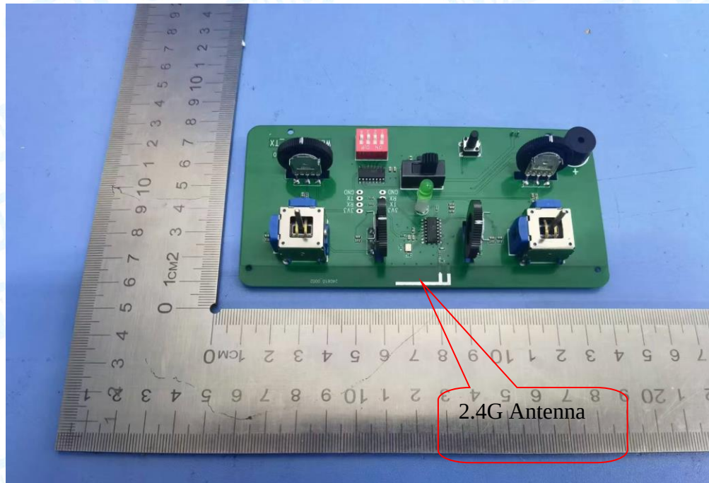
Photo 11 Appearance of PCB
