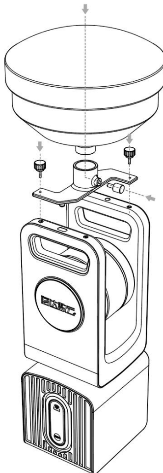
Figure 3-2.5 Installation diagram of HD TLS360 system RTK
