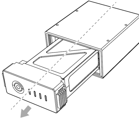
Figure 3-2.2 Battery Disassembly
