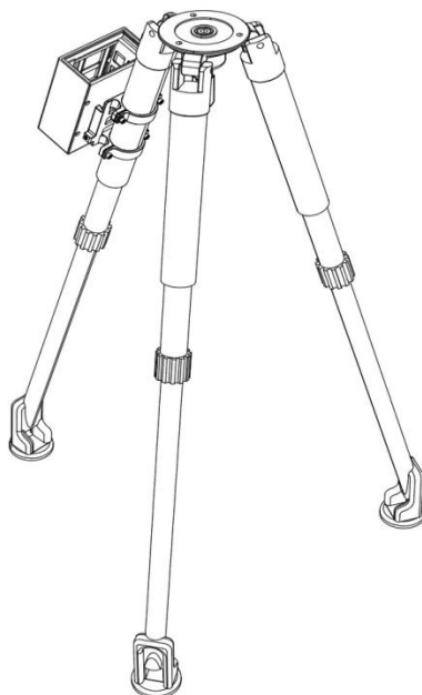
Figure 2-7 HD TLS360 system carbon fiber tripod
