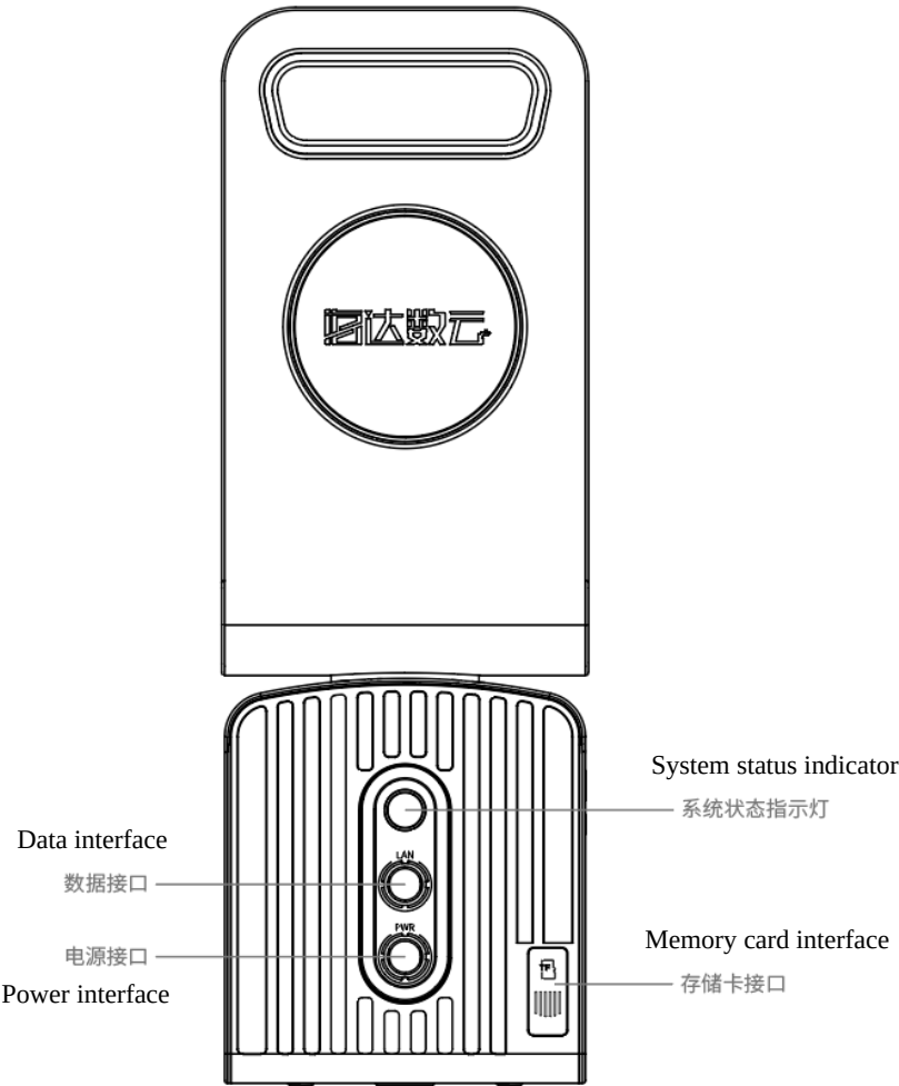
Figure 2-1 Host and interface diagram of HD TLS360 system
