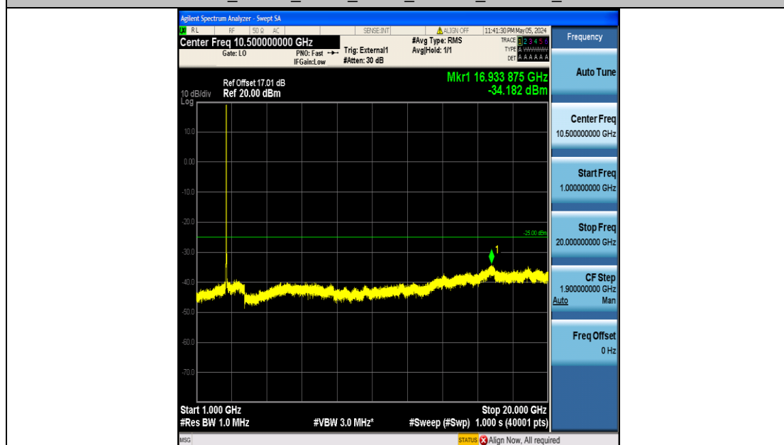
Band38_15MHz_QPSK_38175_75RB#0_1000~20000_1000~20000
