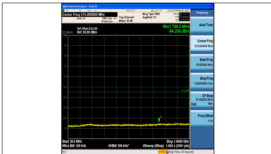
Band38_15MHz_QPSK_38175_75RB#0_30~1000_30~1000
