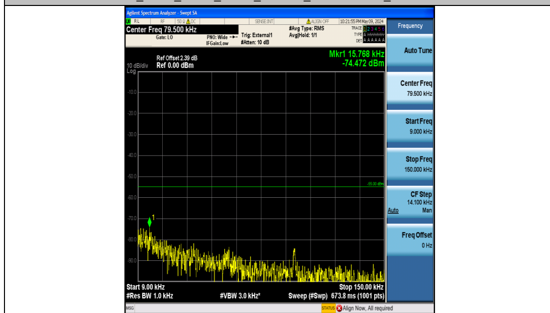
Band41_5MHz_16QAM_40065_25RB#0_0.009~0.15_0.009~0.15
