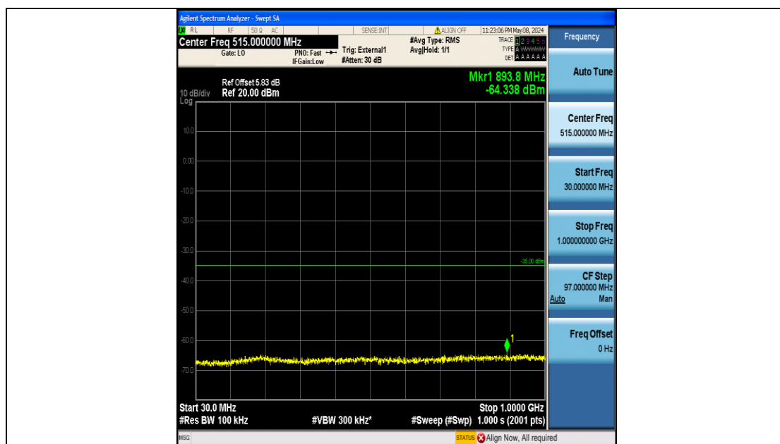
Band41_15MHz_QPSK_41165_75RB#0_30~1000_30~1000
