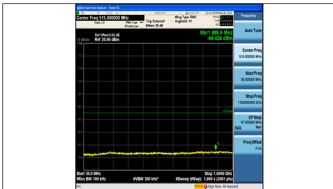
Band41_5MHz_16QAM_40590_25RB#0_30~1000_30~1000
