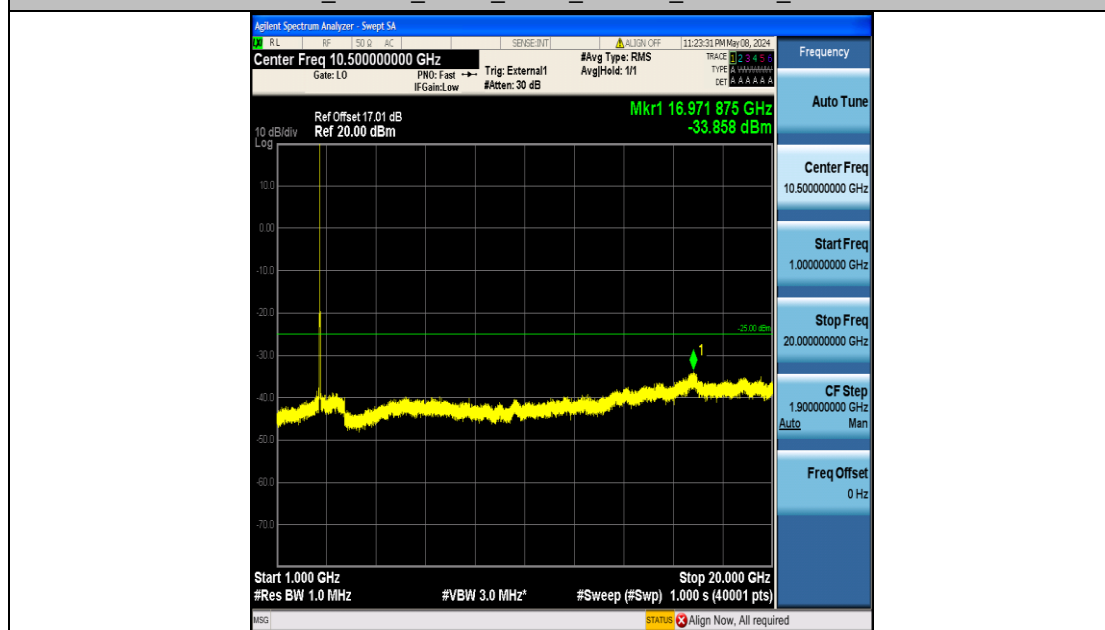
Band41_15MHz_QPSK_41165_75RB#0_1000~20000_1000~20000
