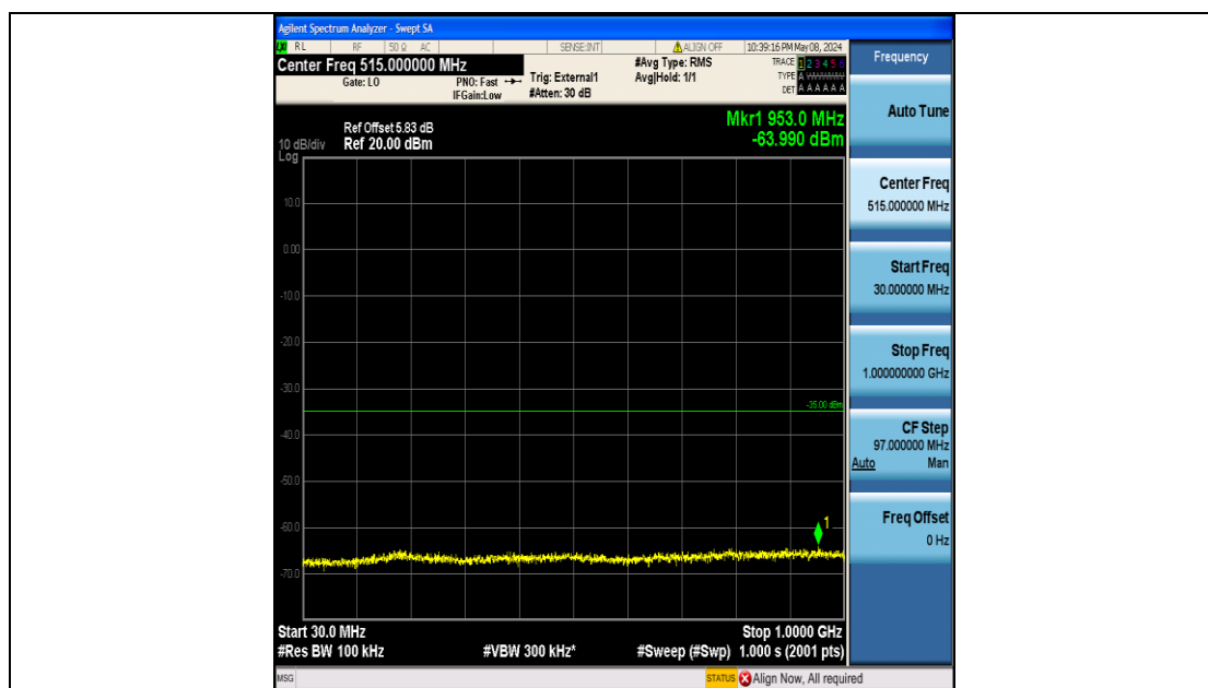
Band41_10MHz_QPSK_41190_50RB#0_30~1000_30~1000
