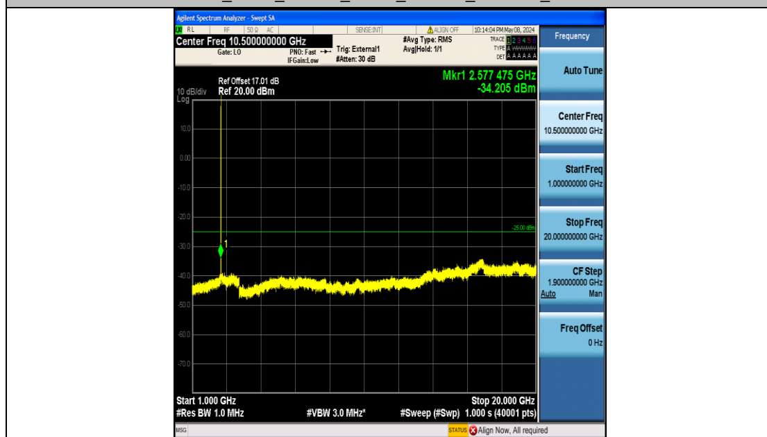
Band41_5MHz_16QAM_40590_25RB#0_1000~20000_1000~20000
