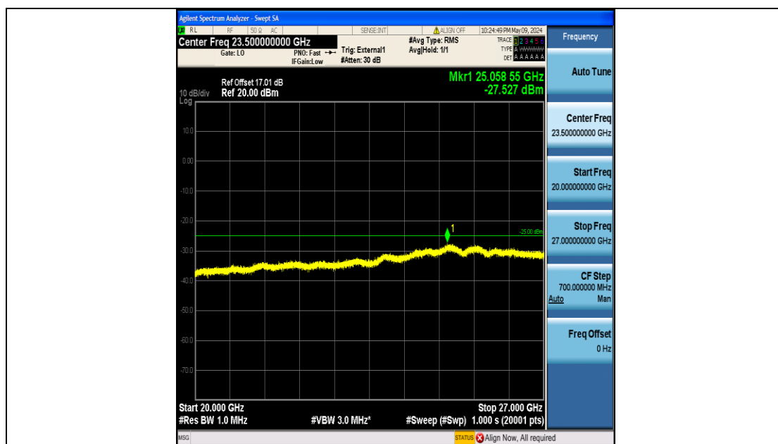
Band41_5MHz_QPSK_41215_25RB#0_20000~27000_20000~27000
