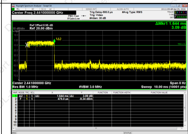
2-DH3
