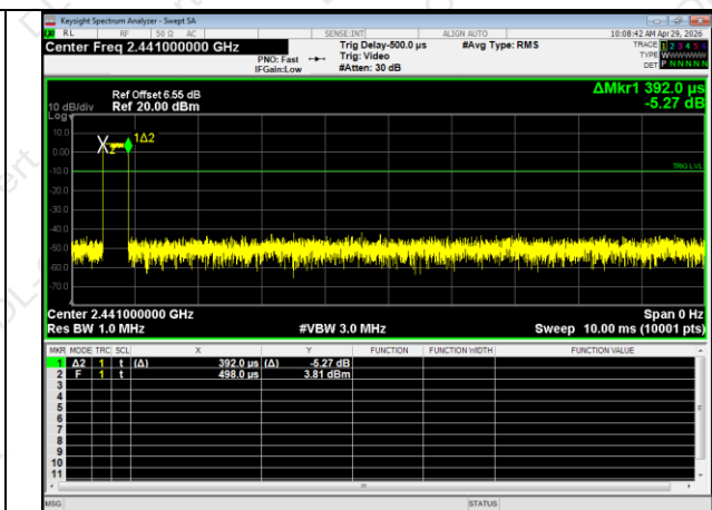
2-DH1
